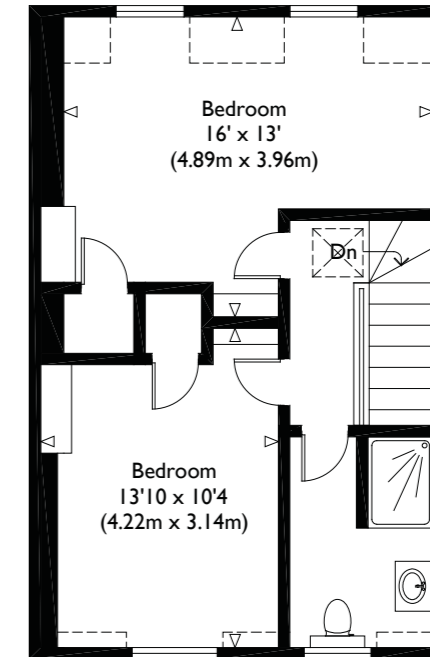
Third Floor
