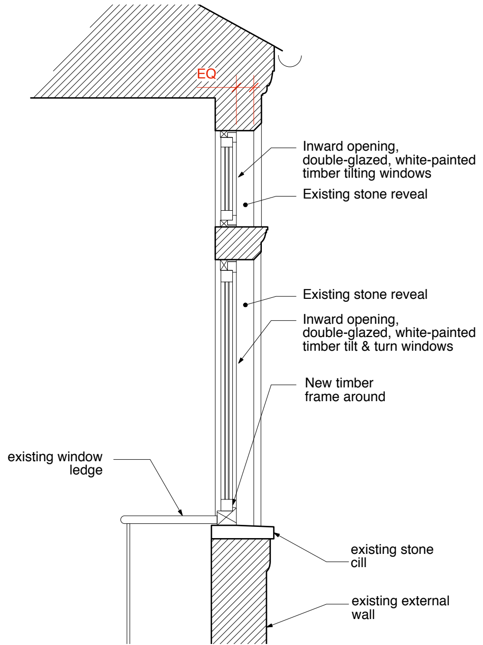
B Section Detail of a Proposed Timber Windows 1:20
