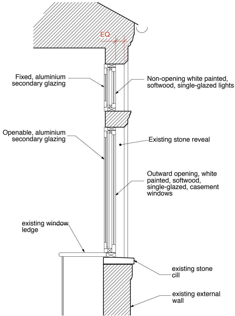
A Typical Section Detail of Existing Casement Window 1:20
