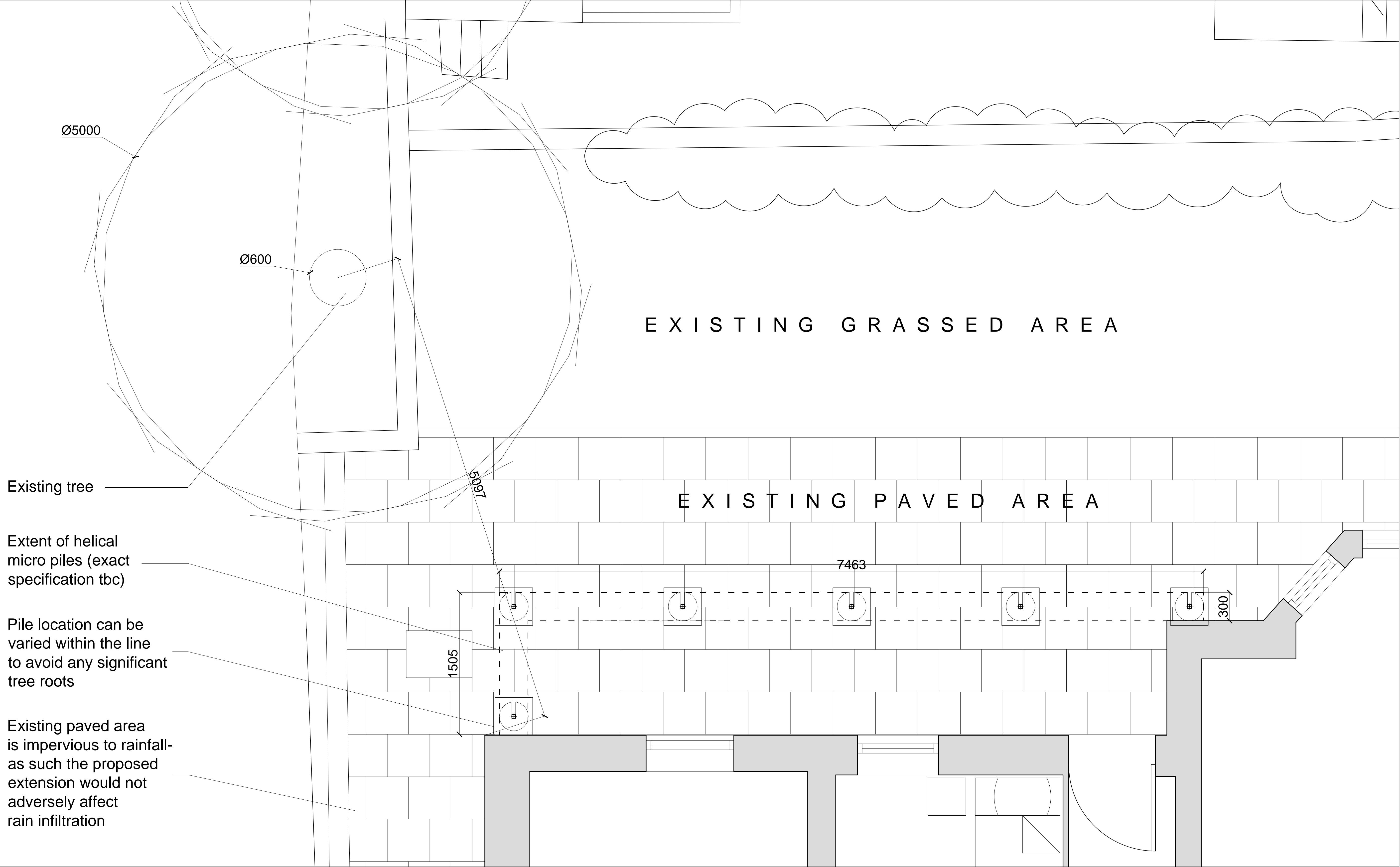
PROPOSED DETAIL PLAN SHOWING HELICAL PILES
