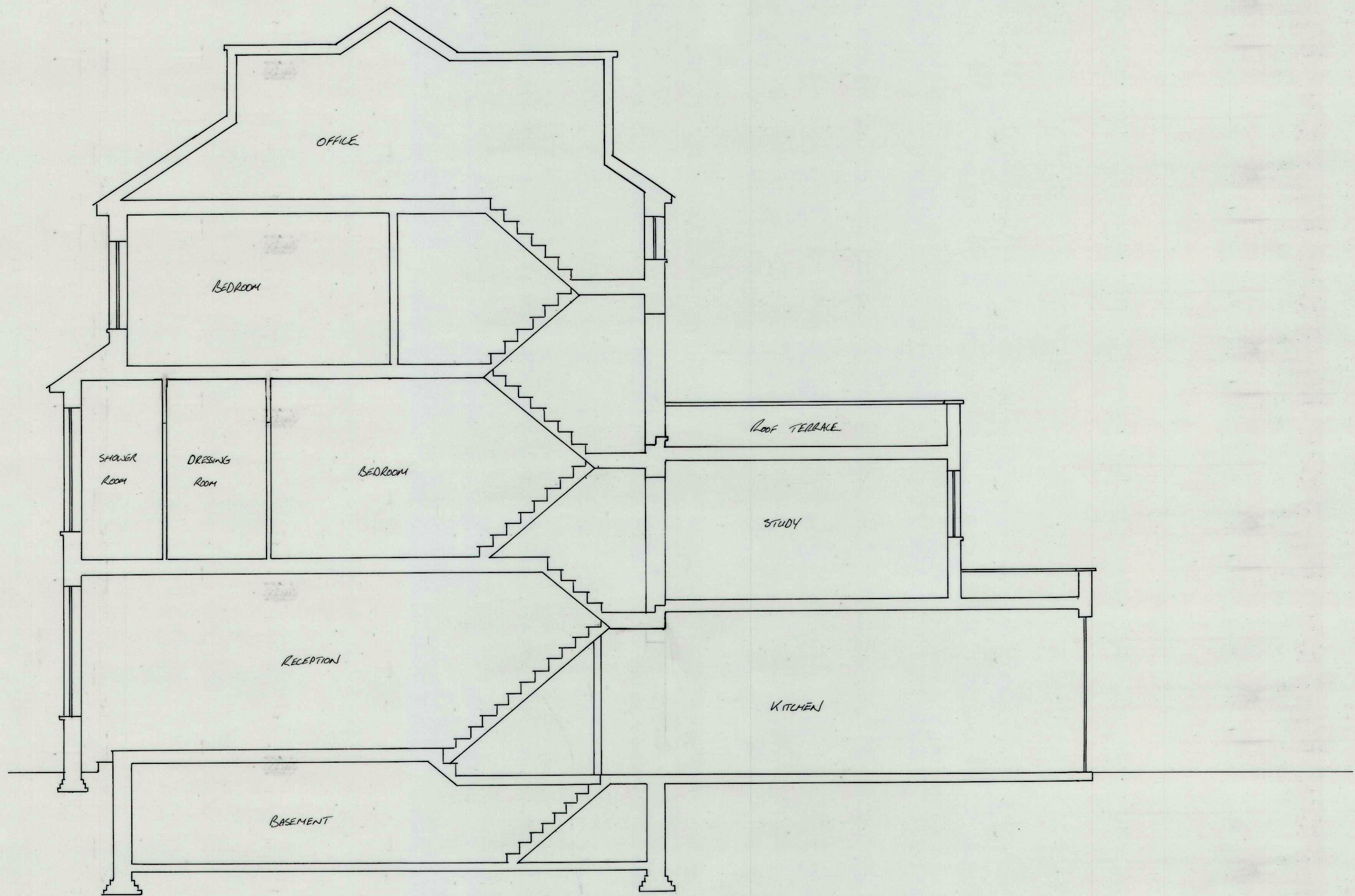
PROPOSED SECTION A-A 1:50
