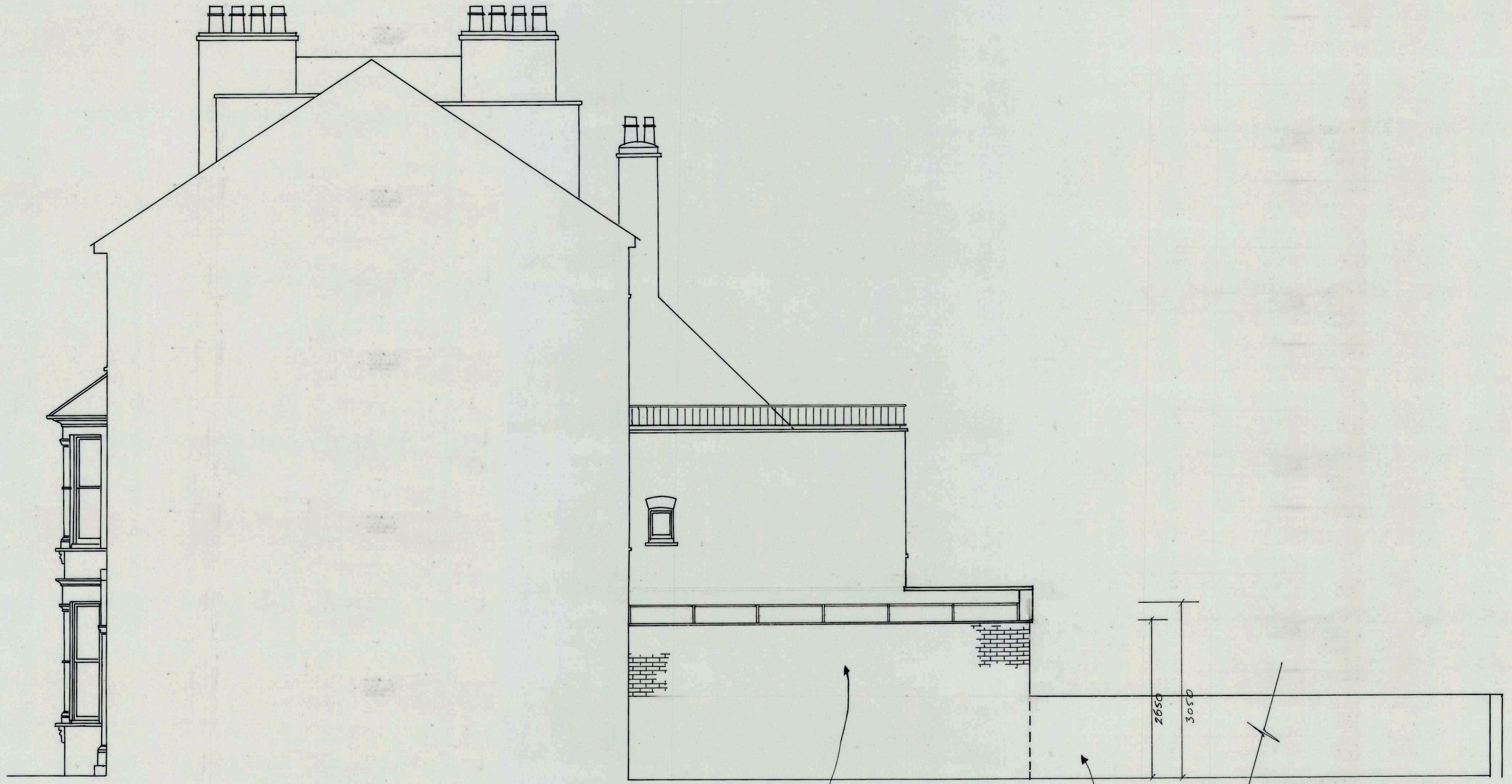
PROPOSED SIDE ELEVATION 1:50
