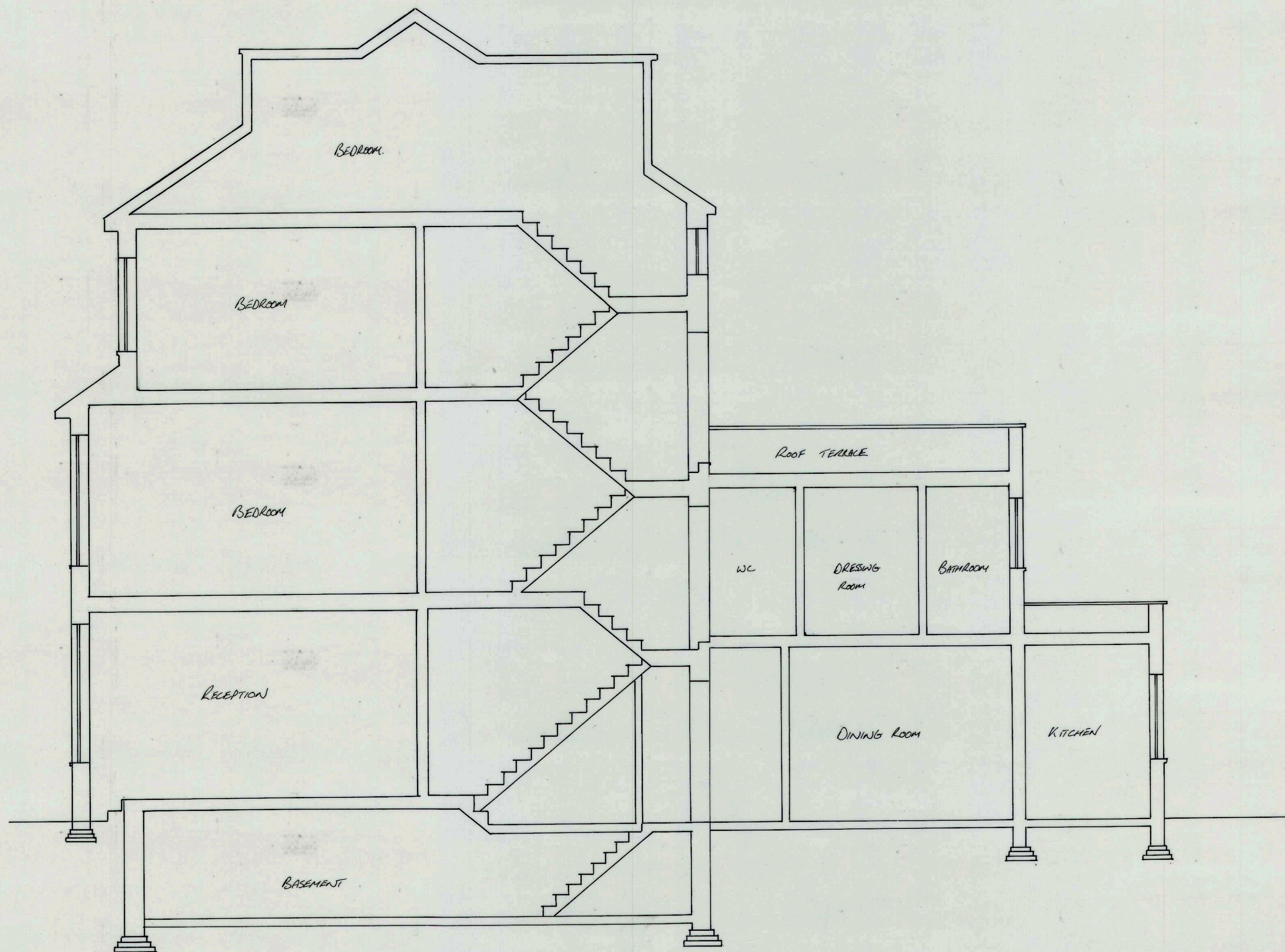
EXISTING SECTION A-A
