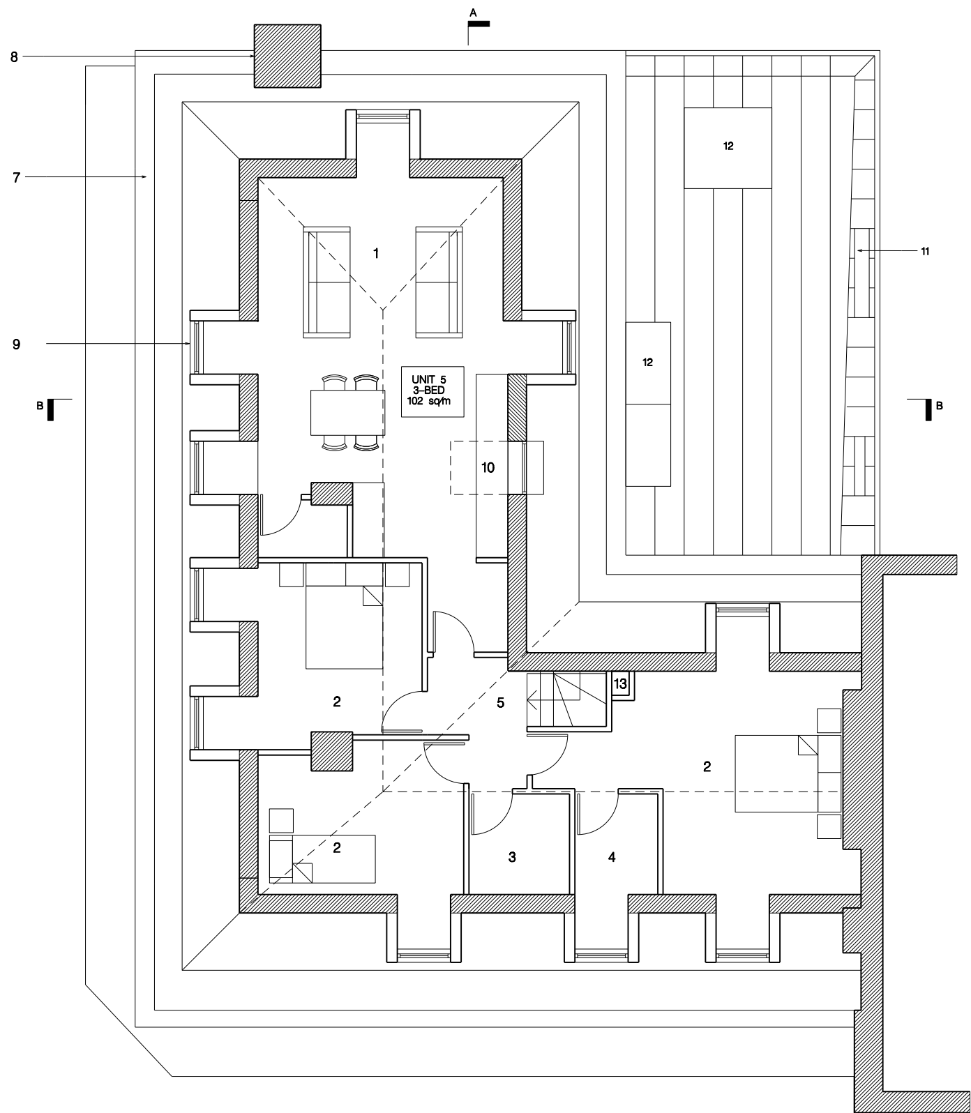
01 PROPOSED THIRD FLOOR PL117 Scale 1:100 @ A3
