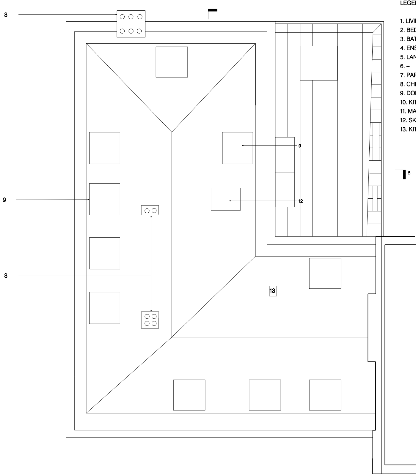
02 PROPOSED ROOF PLAN PL117 Scale 1:100 @ A3
