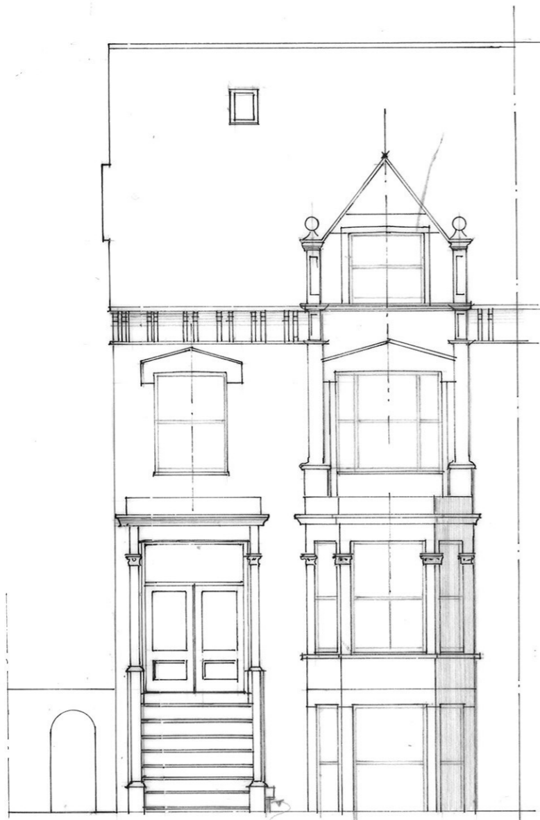
FRONT ELEVATION.
