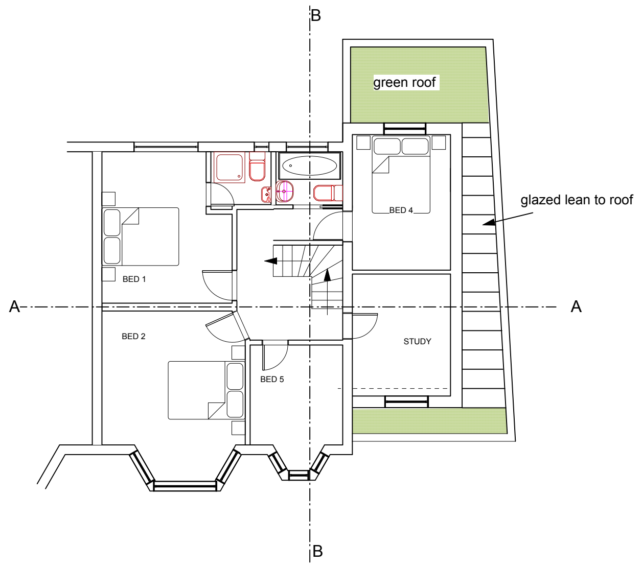
1st Floor
