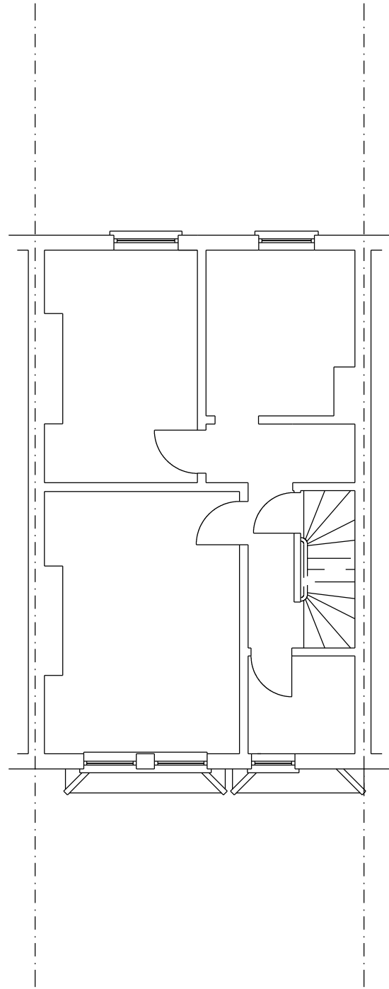
SECOND FLOOR
