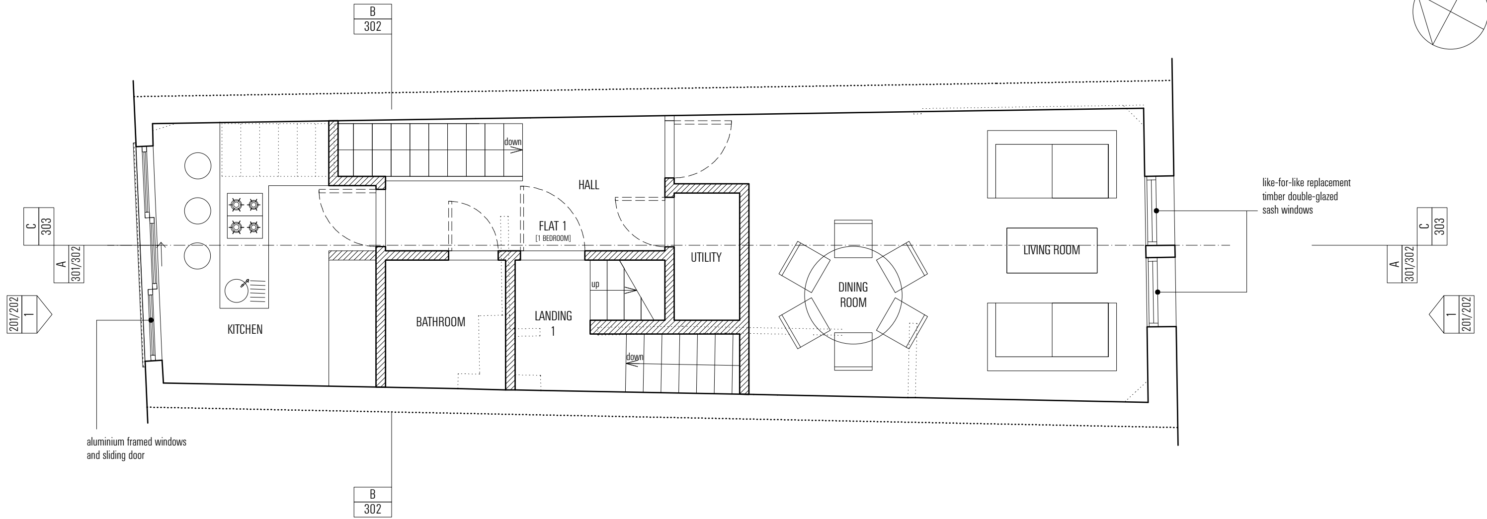
1ST FLOOR PLAN
