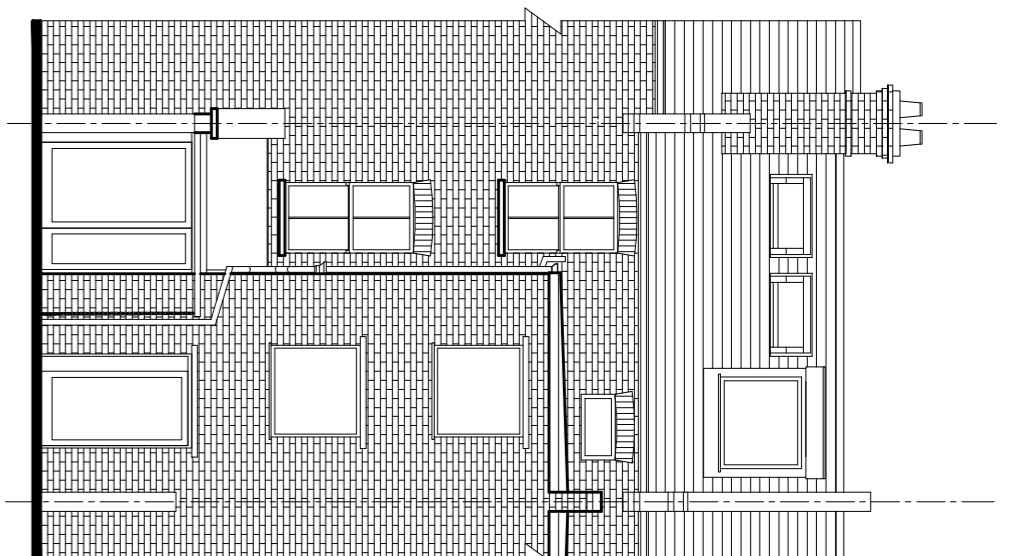
REAR ELEVATION AS PROPOSED
