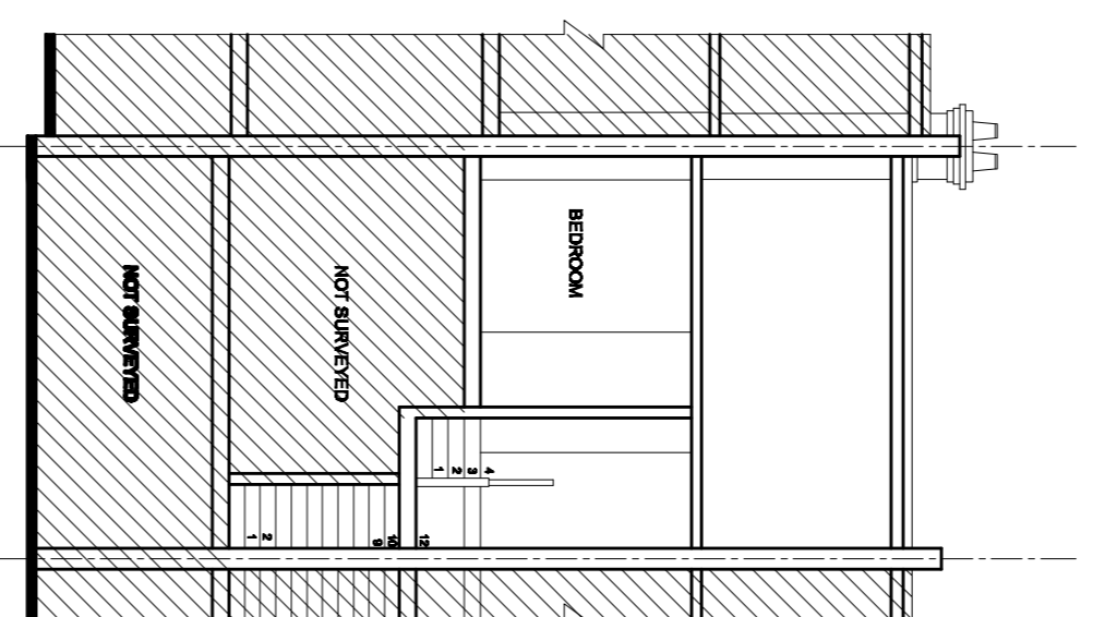
CROSS SECTION AS EXISTING
