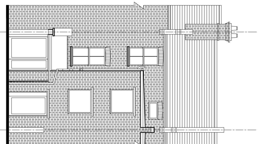
REAR ELEVATION AS EXISTING
