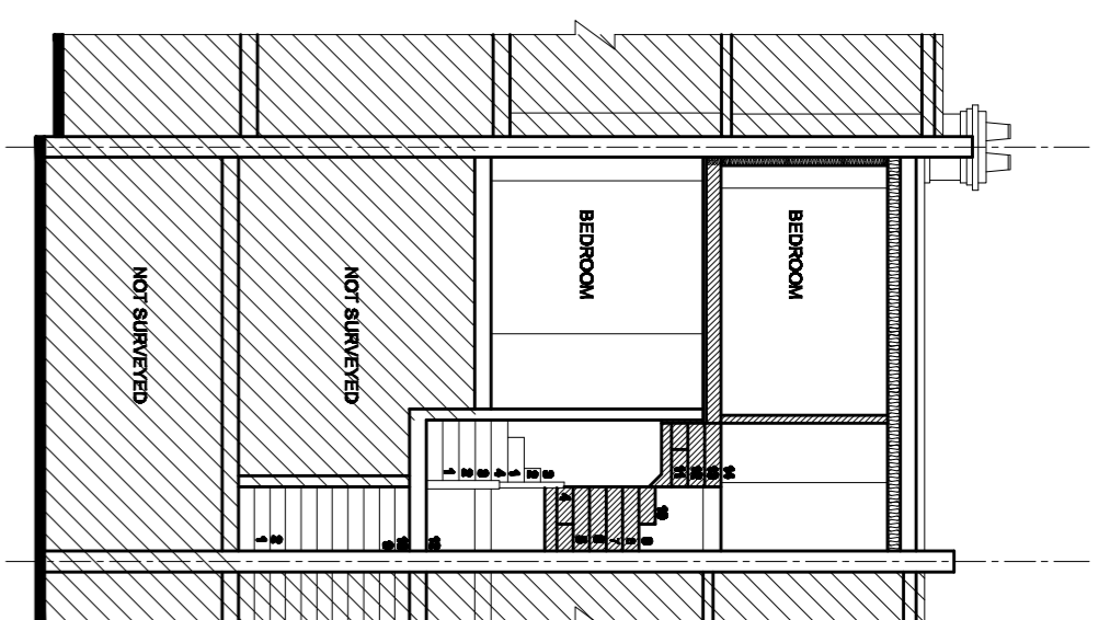
CROSS SECTION AS PROPOSED
