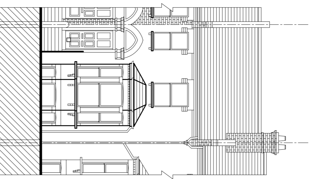
FRONT ELEVATION AS EXISTING
