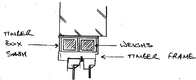
MULLION DETAIL (1:10)
