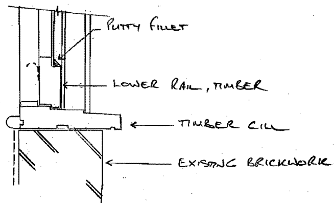
LOWER CILL (1:10)
