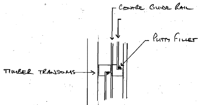
CENTRE RAIL (1:10)
