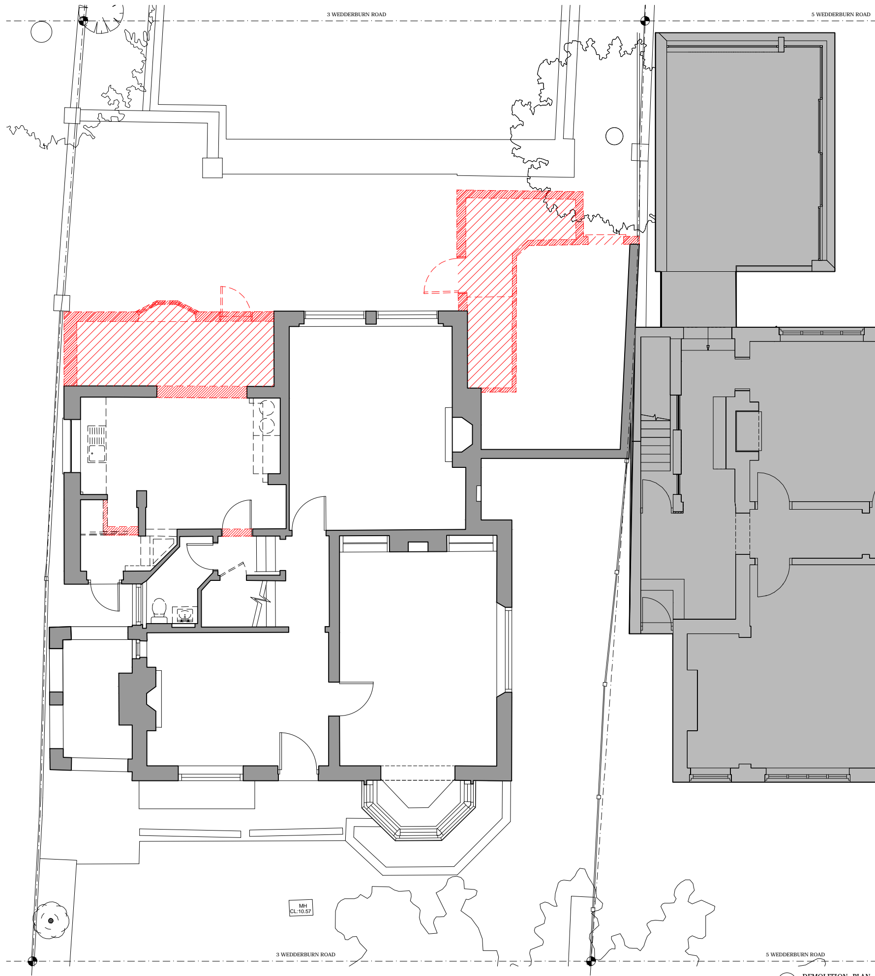
1 DEMOLITION PLAN 1:50@A1/ 1:100@A3
