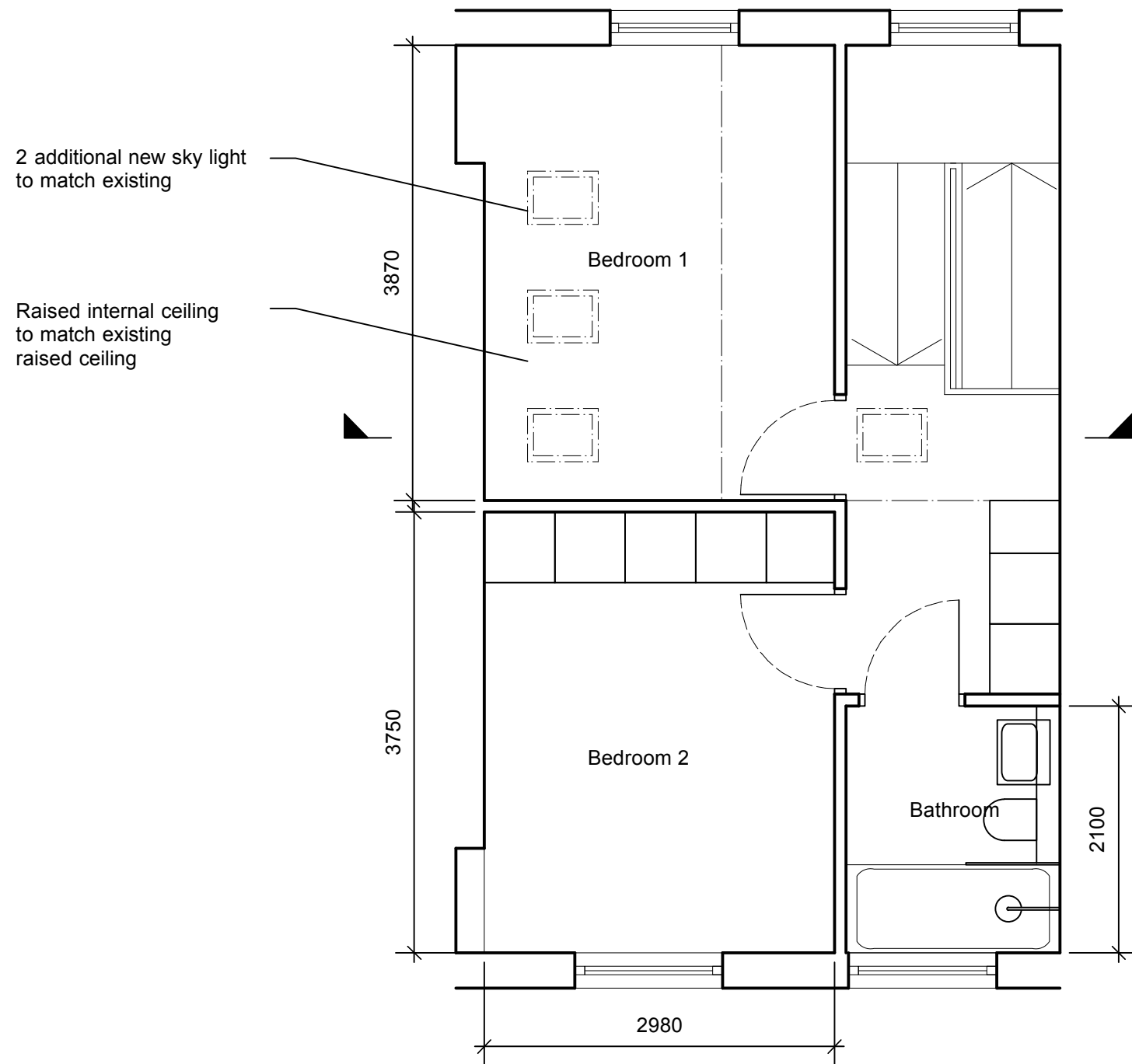
TOP FLOOR PLAN
