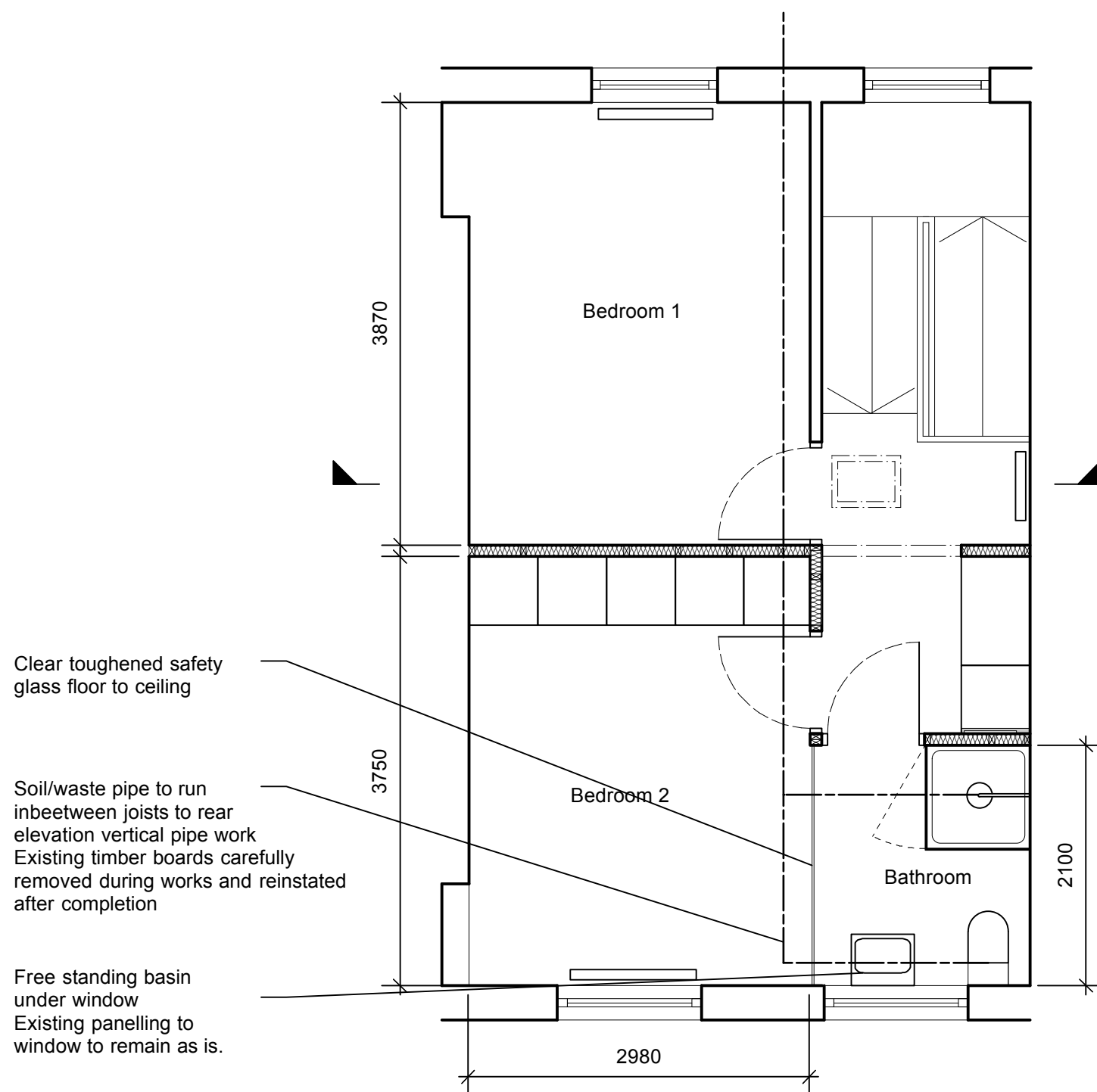
TOP FLOOR PLAN
