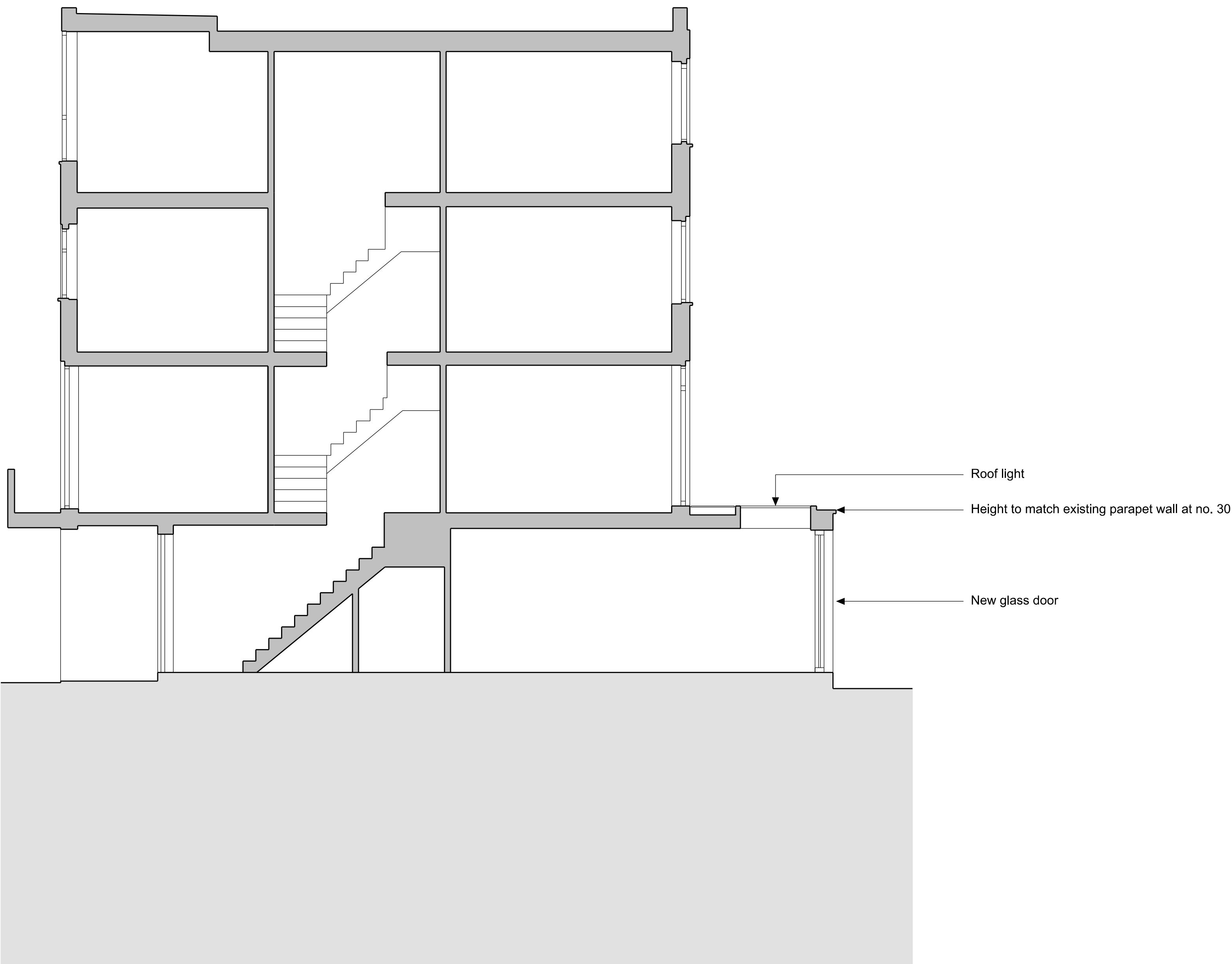
01 Proposed Section AA Scale 1:50 @A1 / 1:100 @A3
