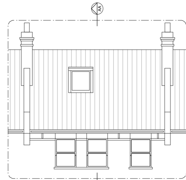
03 Section BB Front Elevation
