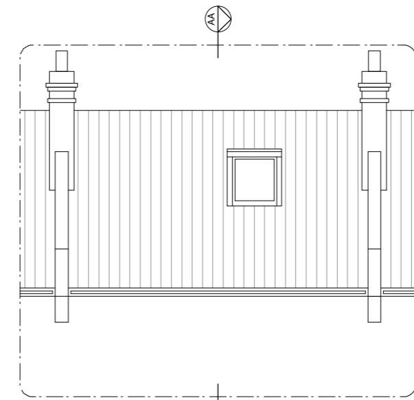
03 Section CC Rear Elevation
