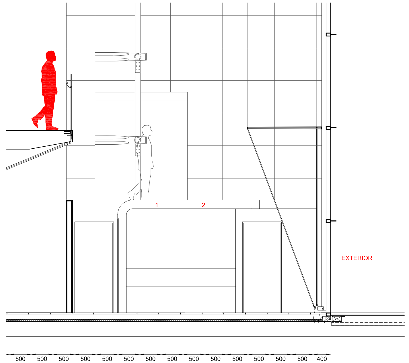
PROPOSED SECTION BB' TRITON SQUARE E:1/100
