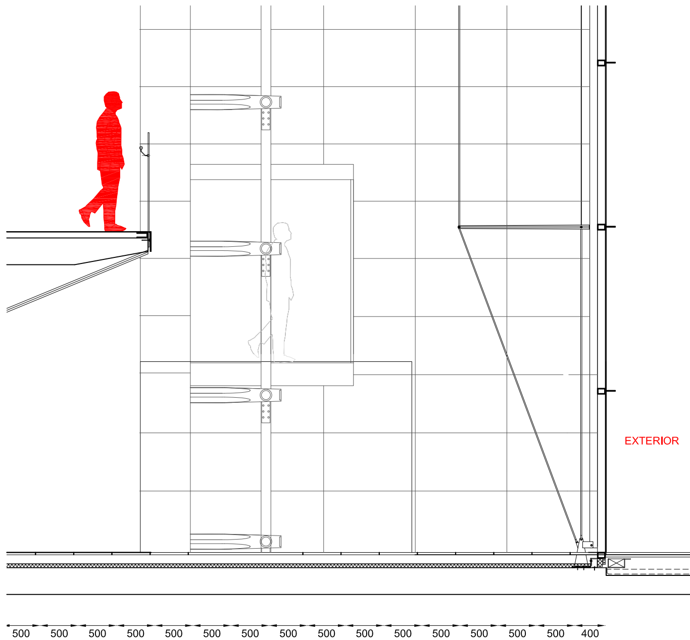
EXISTING SECTION BB' TRITON SQUARE E:1/100
