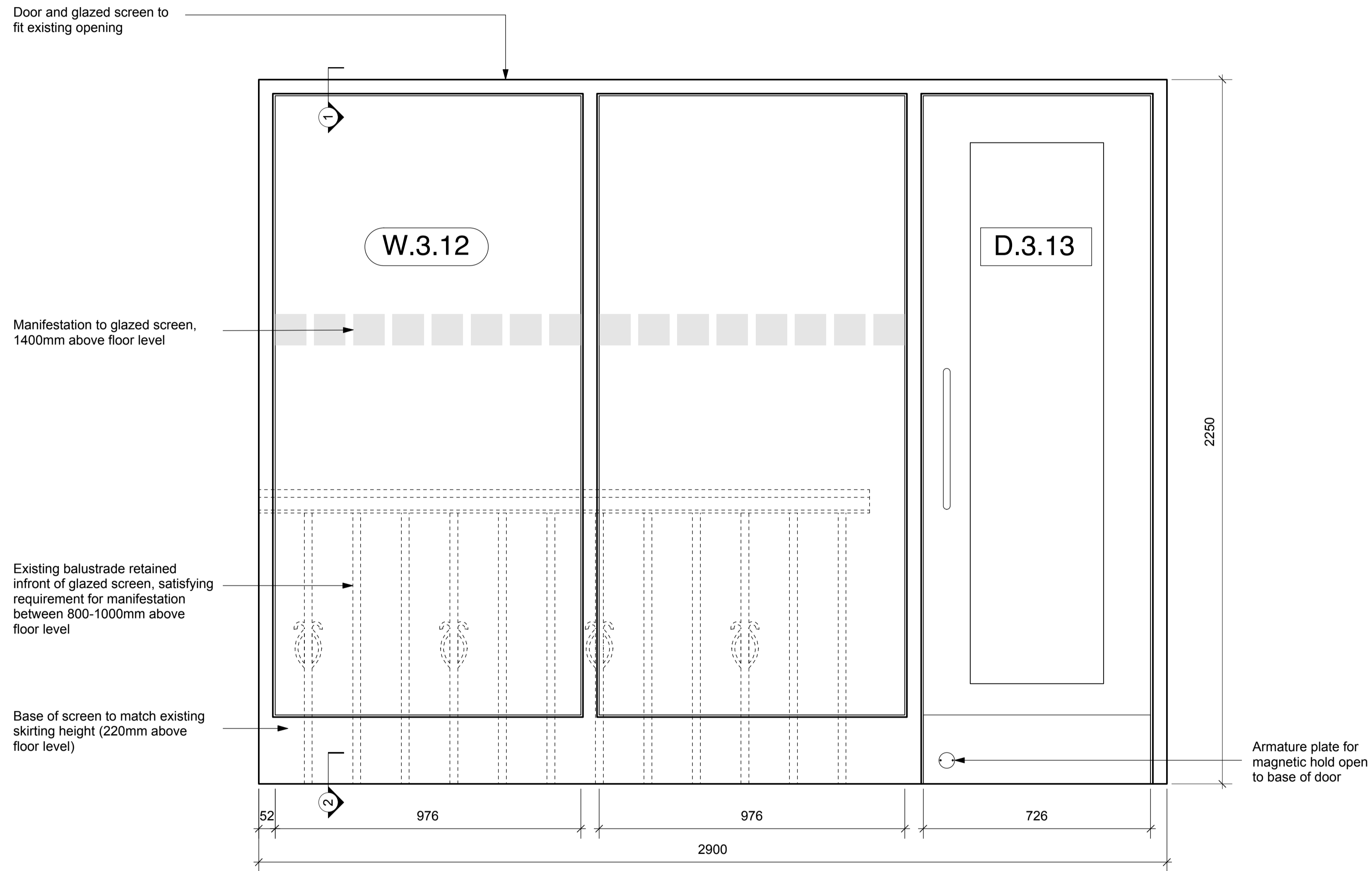
Glazed Screen Elevation scale 1:10
