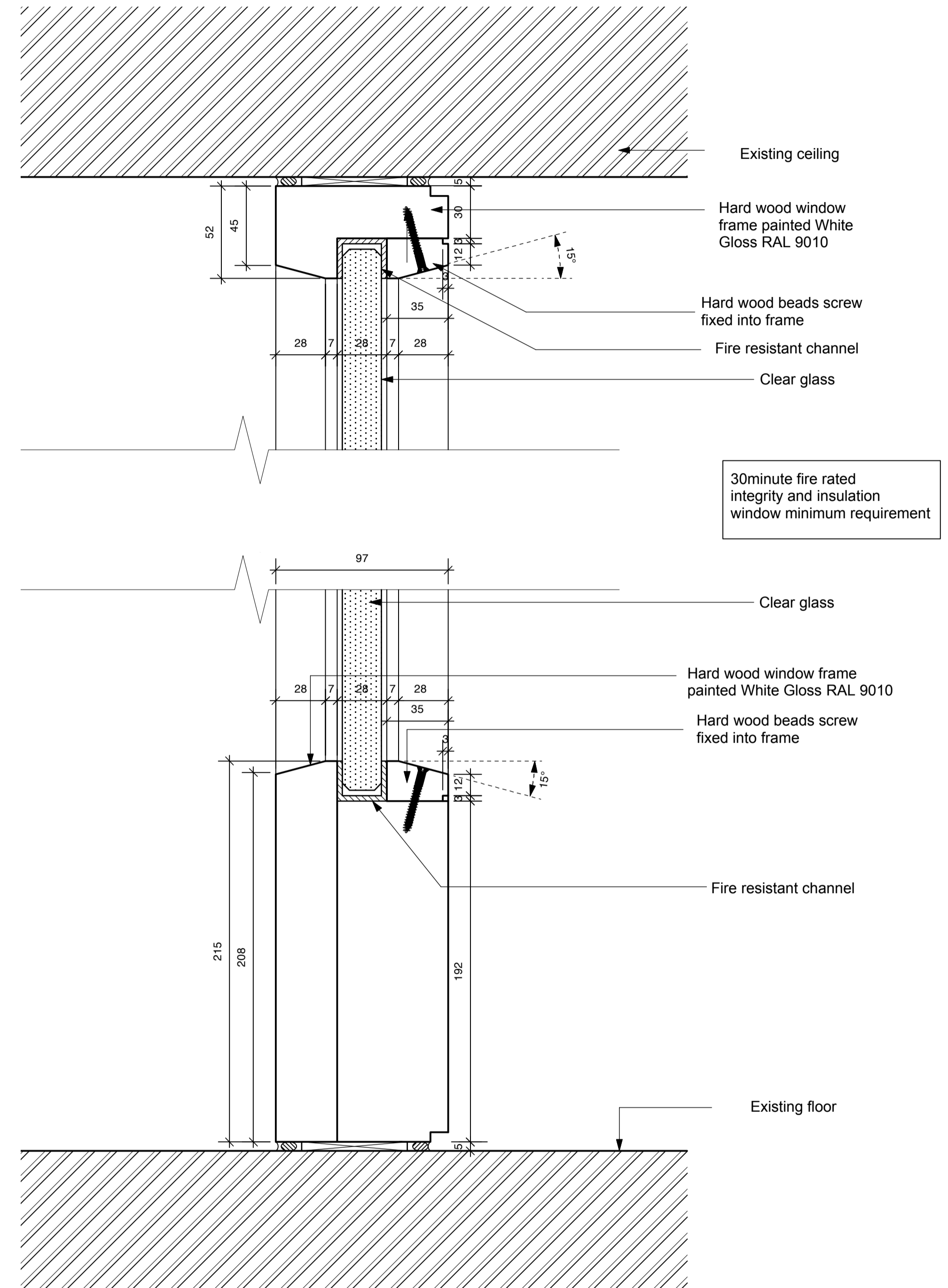
2 Glazed Screen Sill Detail scale 1:2
