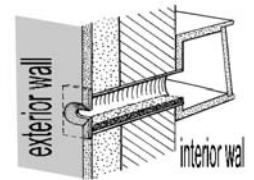
Cutaway: Installation (View from outside building)
