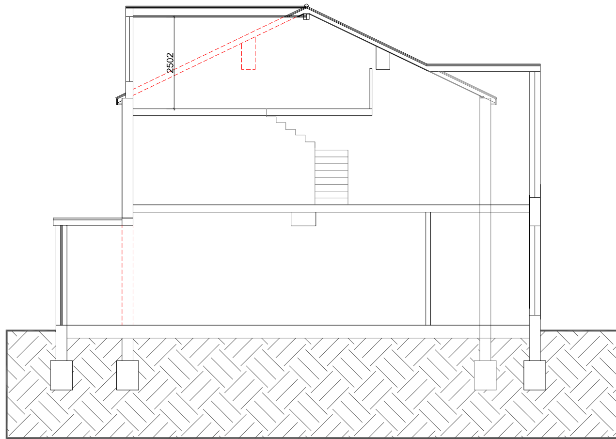
SECTION C-C
