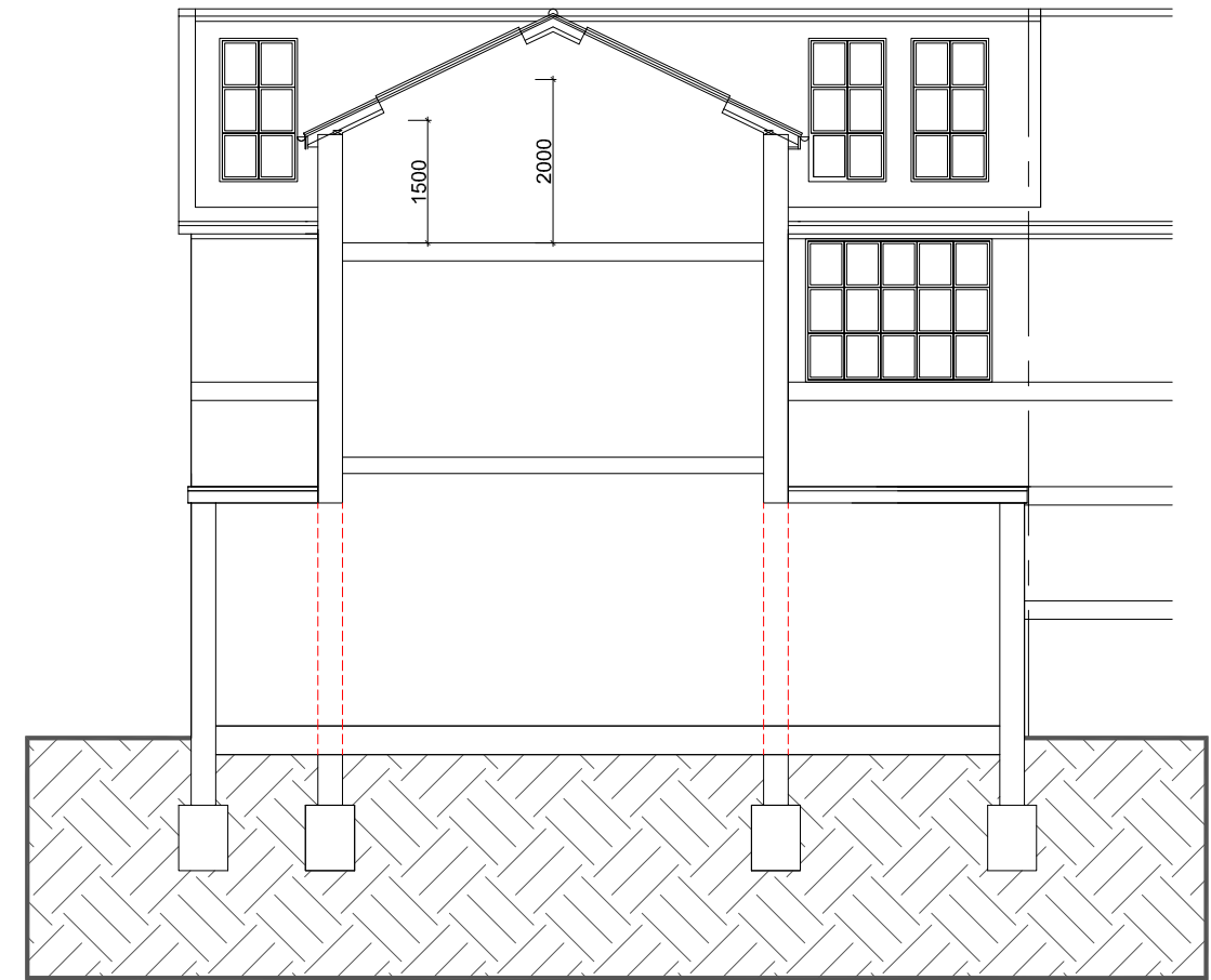
SECTION E-E
