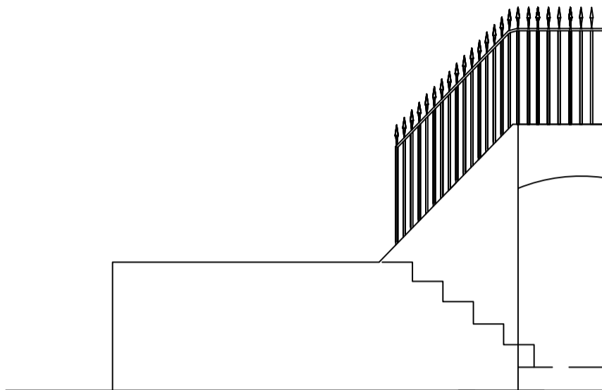
Existing front-side elevation
