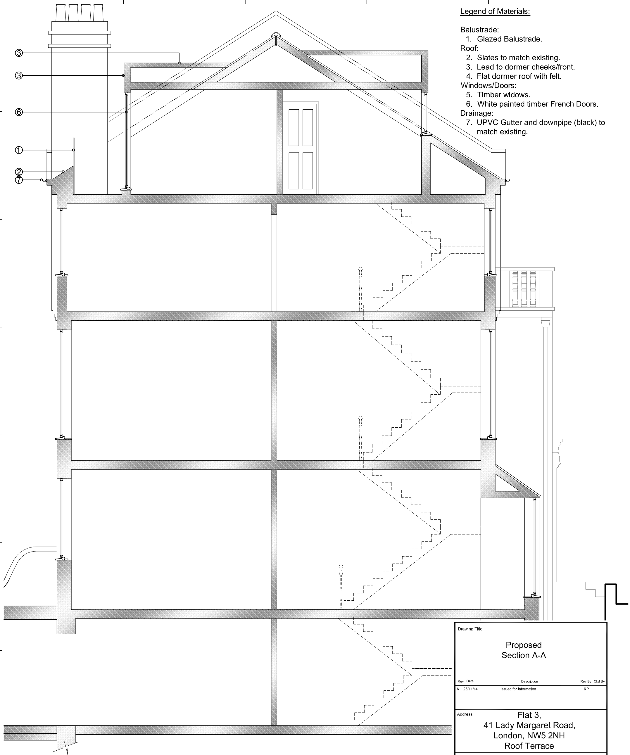
7A PROPOSED SECTION A-A SCALE 1:50
