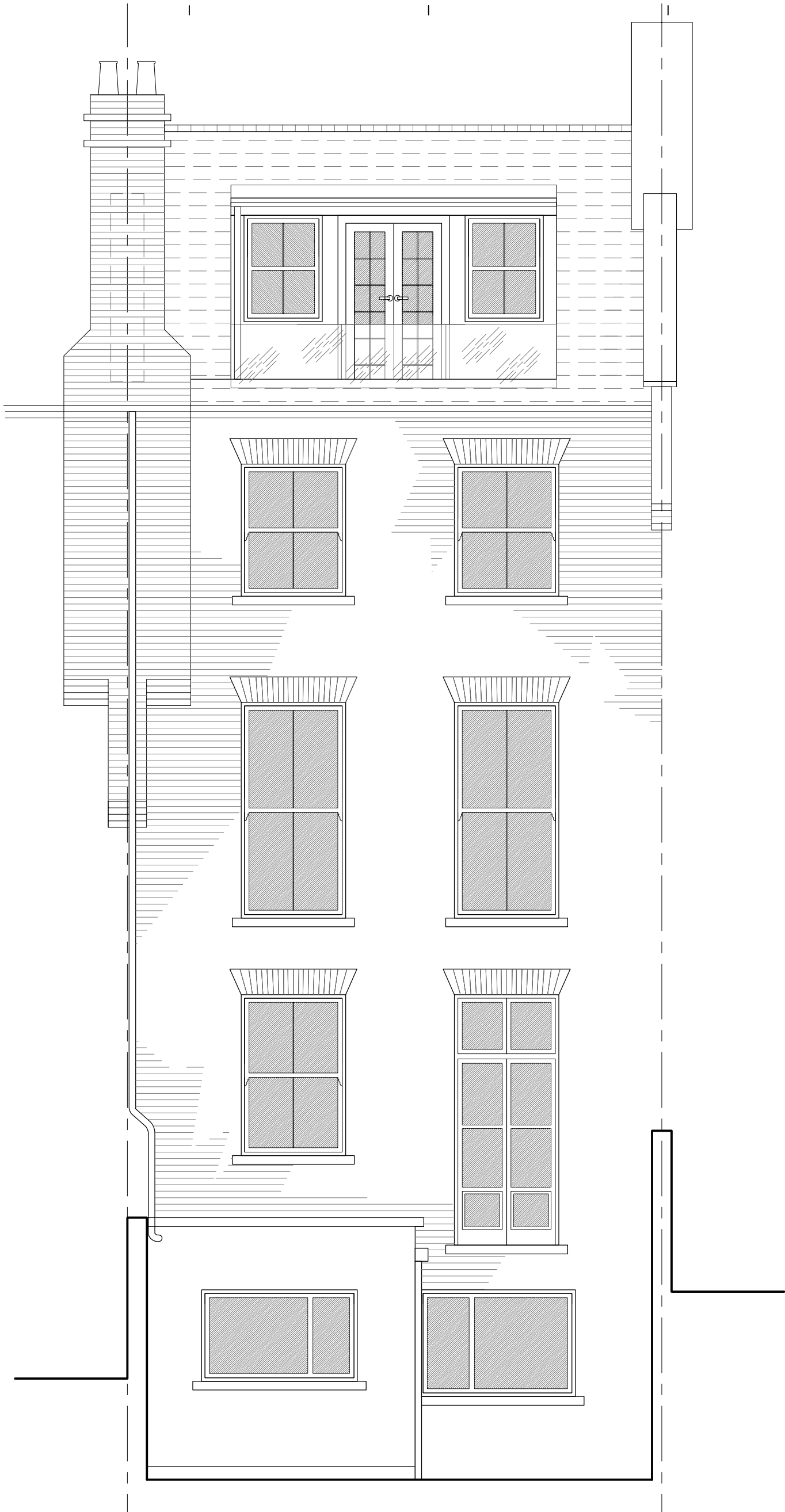
4A PROPOSED REAR ELEVATION
