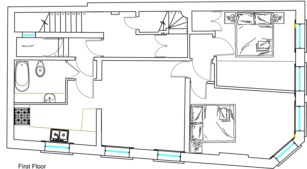
First Floor Scale: 1/100
