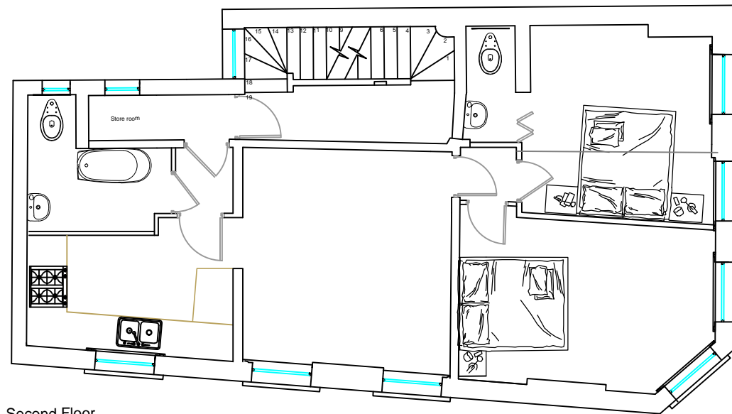
Second Floor Scale: 1/100
