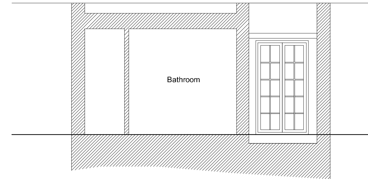
SECTION BB
