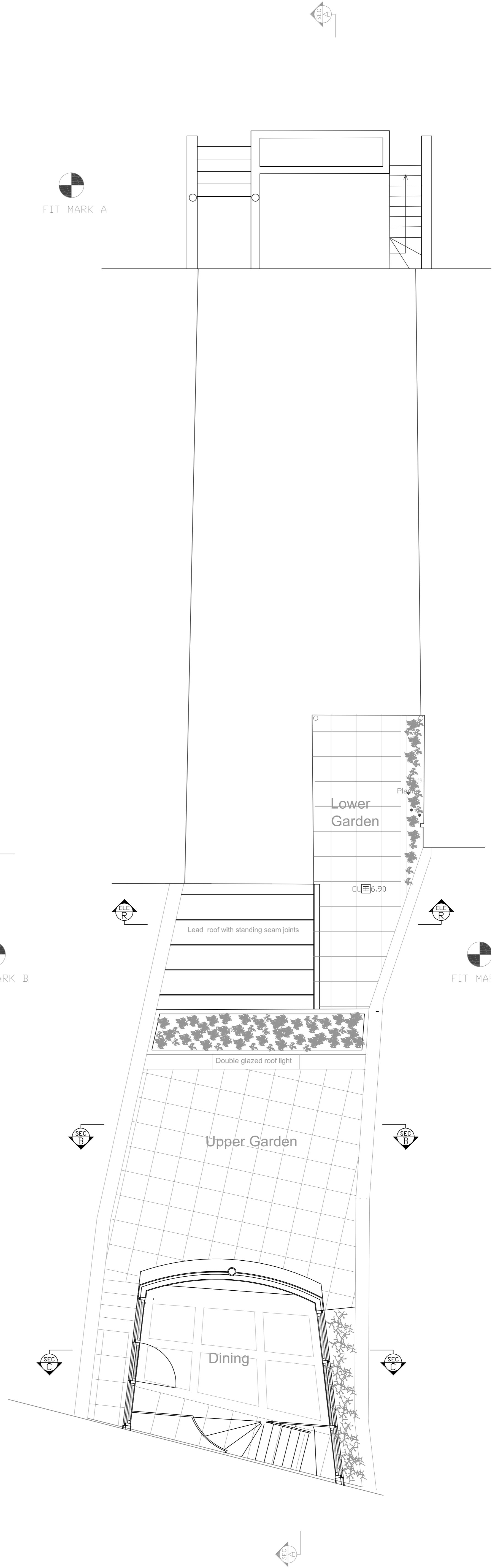
Upper Garden level Plan as Proposed 1:50
