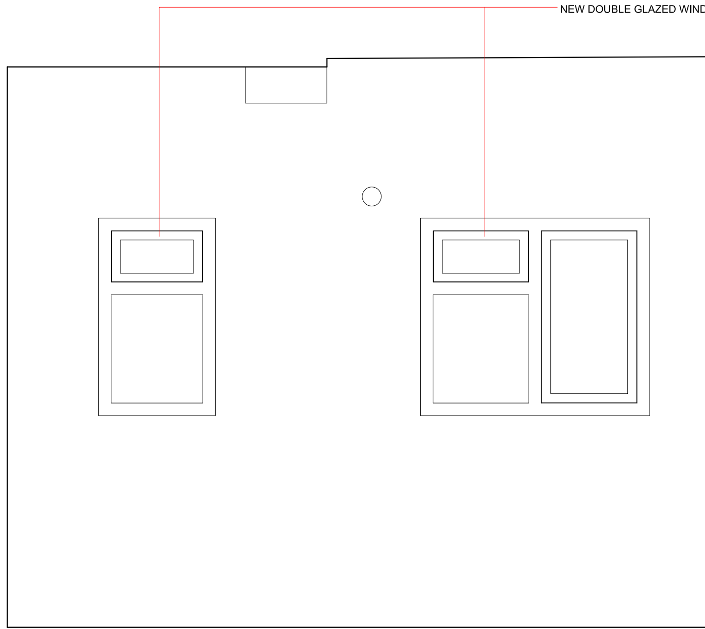
1 PROPOSED ELEVATION AA SCALE 1:20 @ A3
