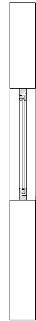
2 PROPOSED WINDOW SECTION SCALE 1:20 @ A3
