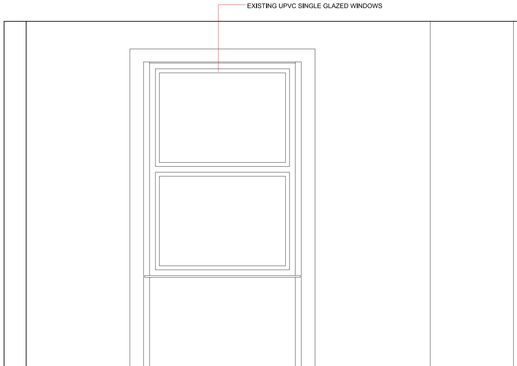
1 EXISTING ELEVATION BB_SECTION 1 SCALE 1:20 @ A3
