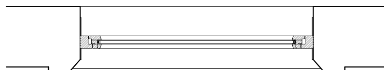
3 EXISTING WINDOW SECTIONS SCALE 1:20 @ A3
