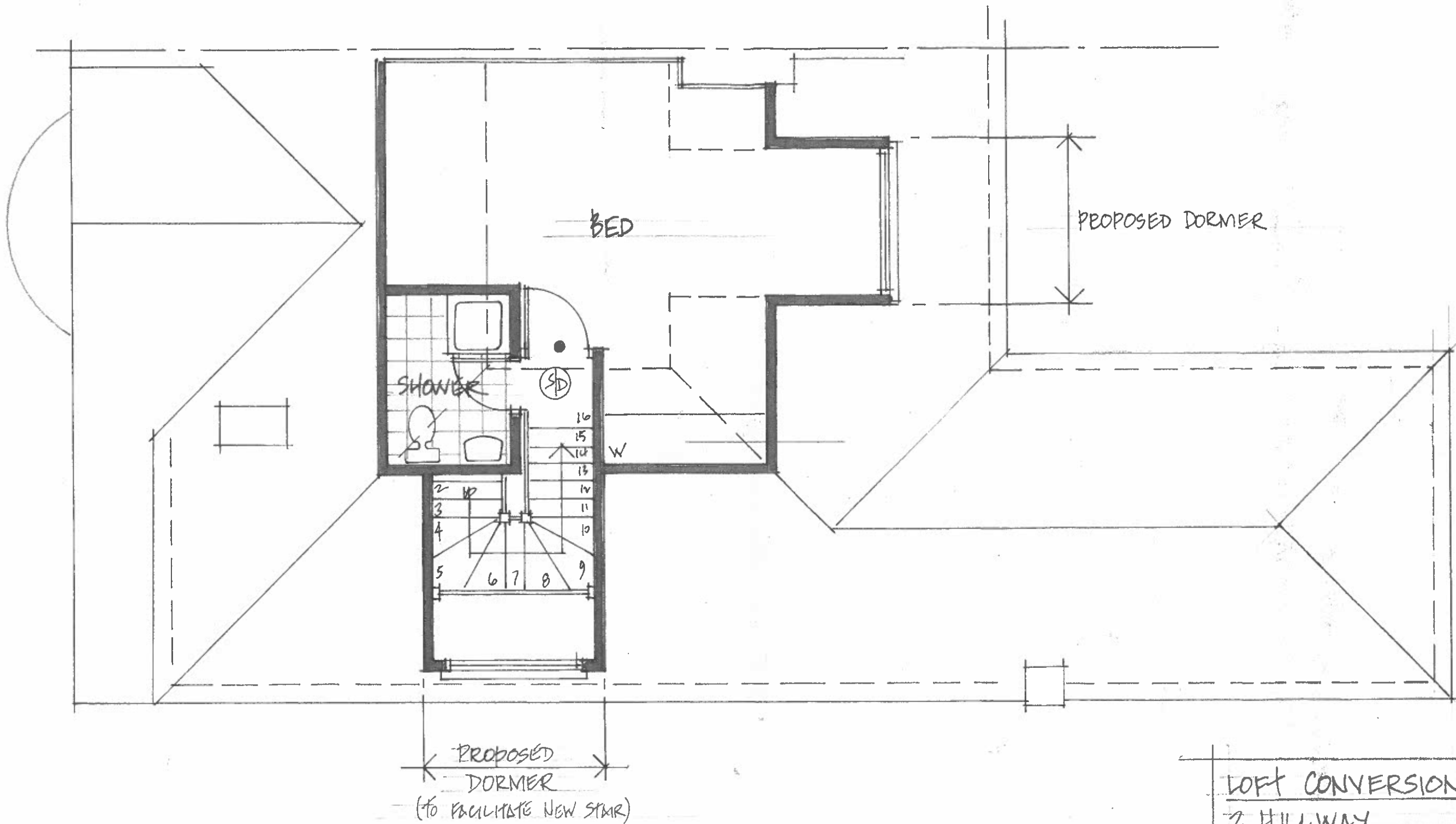
PROPOSED SECOND FLOOR PLAN - 1:50
