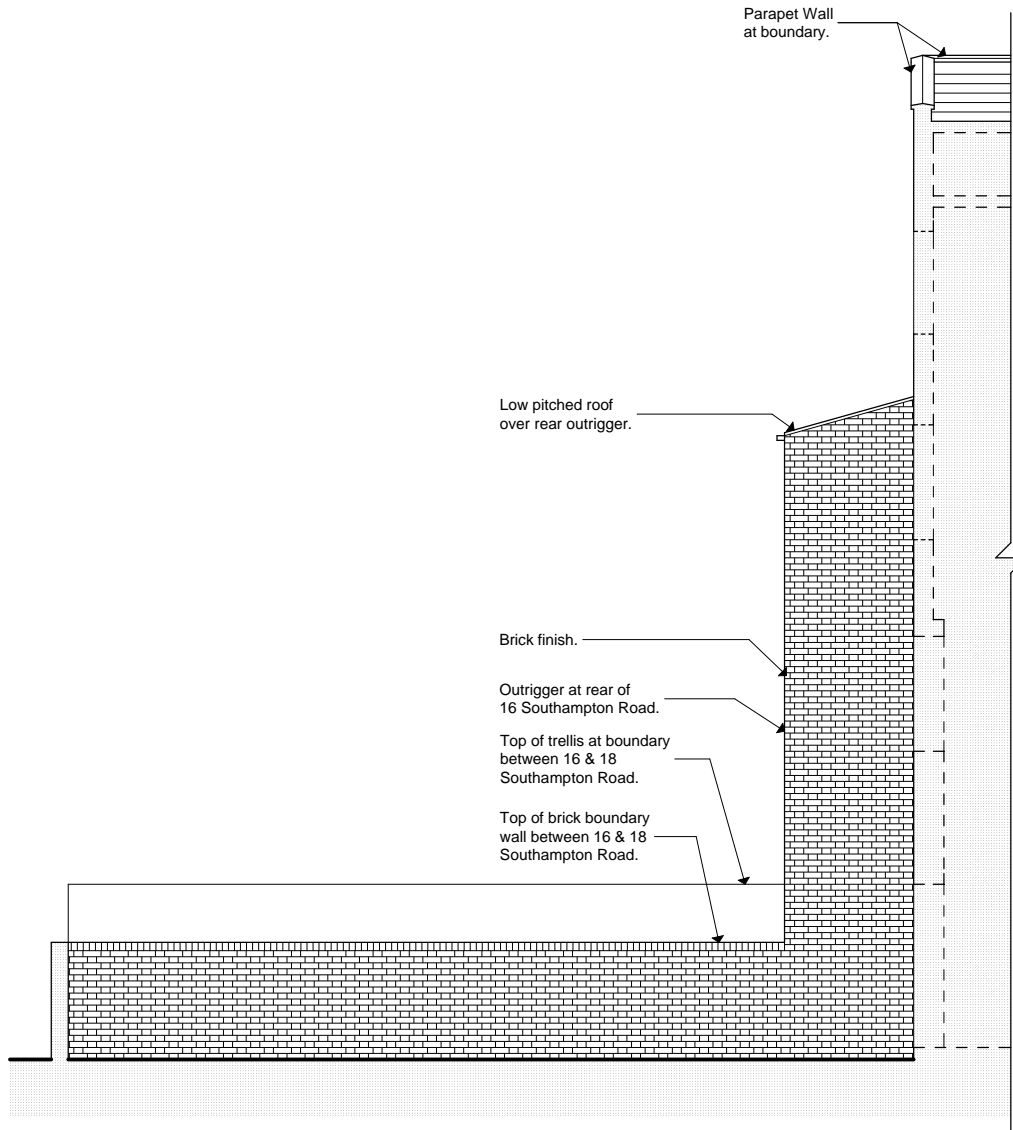
Existing Section A-A (Through 18 Southampton Road)
