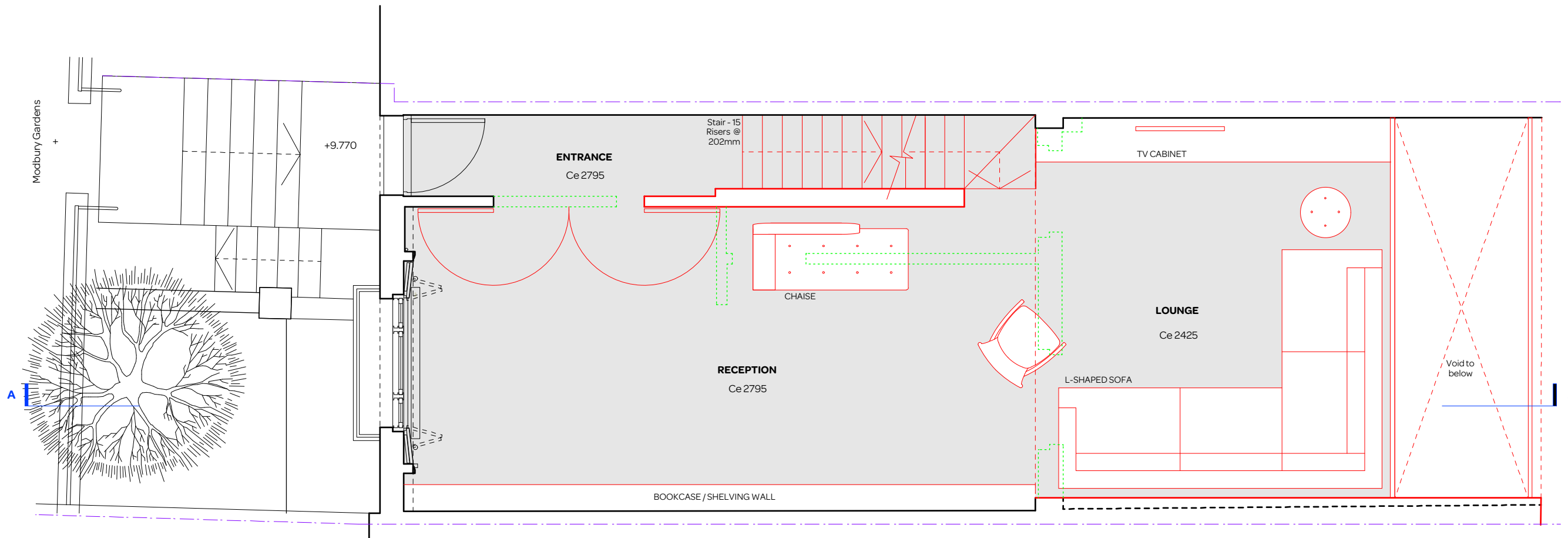
PROPOSED RAISED GROUND FLOOR PLAN
