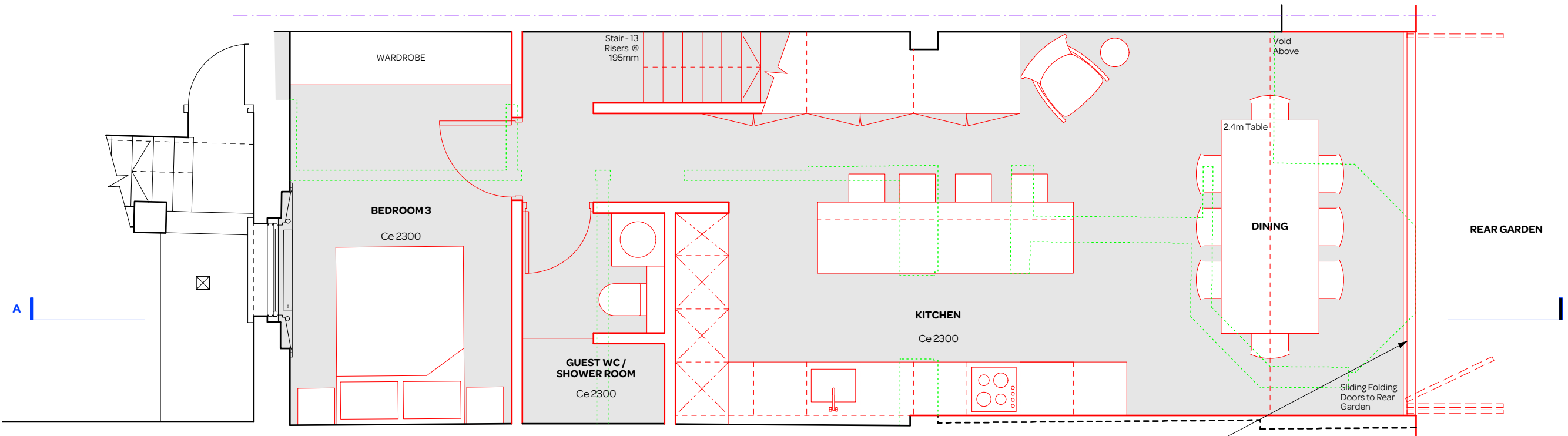
PROPOSED LOWER GROUND FLOOR PLAN
