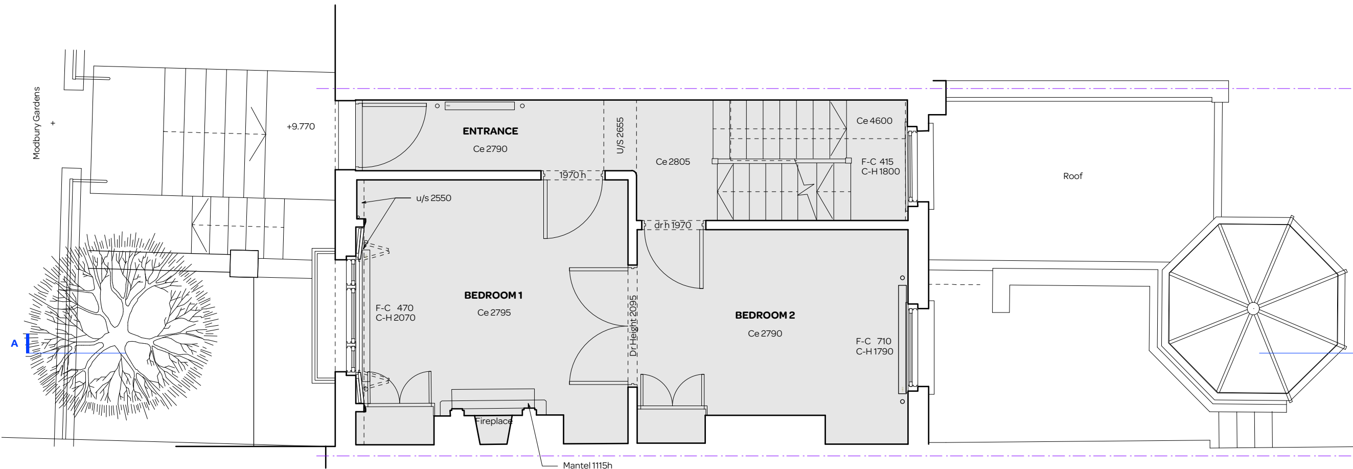
EXISTING RAISED GROUND FLOOR PLAN
