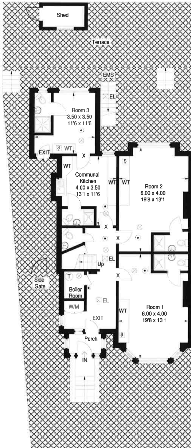
Ground Floor
