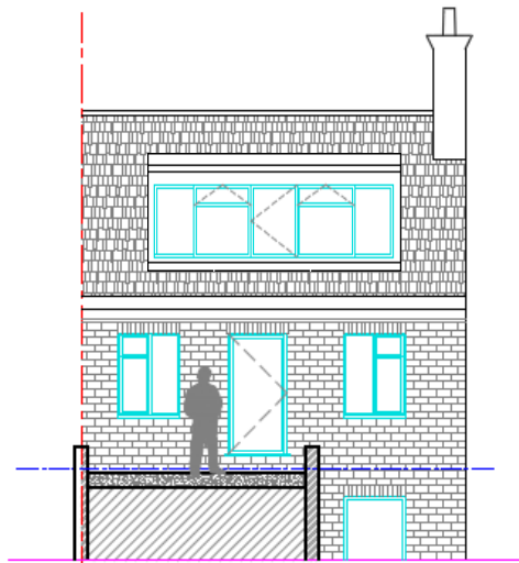
Approved Proposal App ref: 2012/4513/P Rear Elevation
