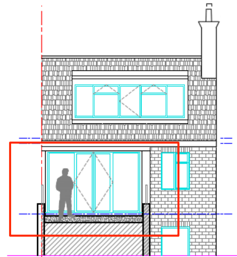
Proposed Rear Elevation 1 of 2 Revision B
