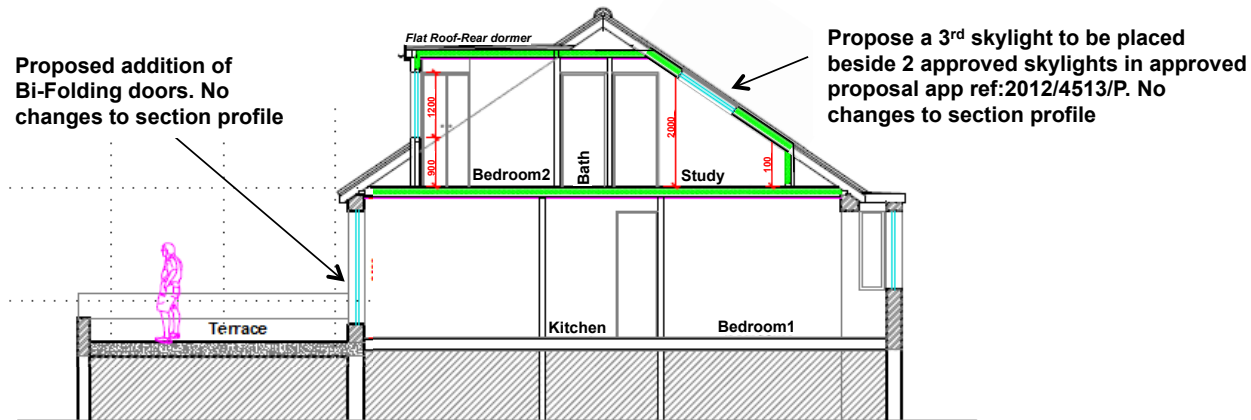
Proposed Section 1 of 2 Revision B
