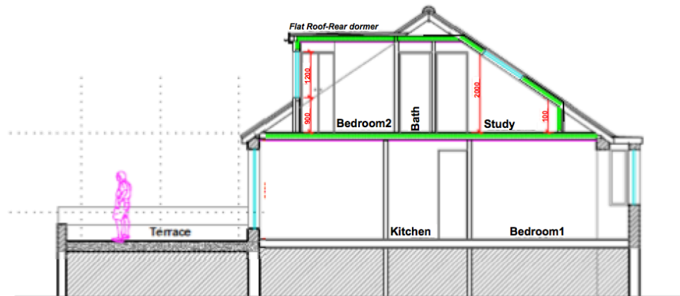
Approved Proposal App ref: 2012/4513/P Section A-A
