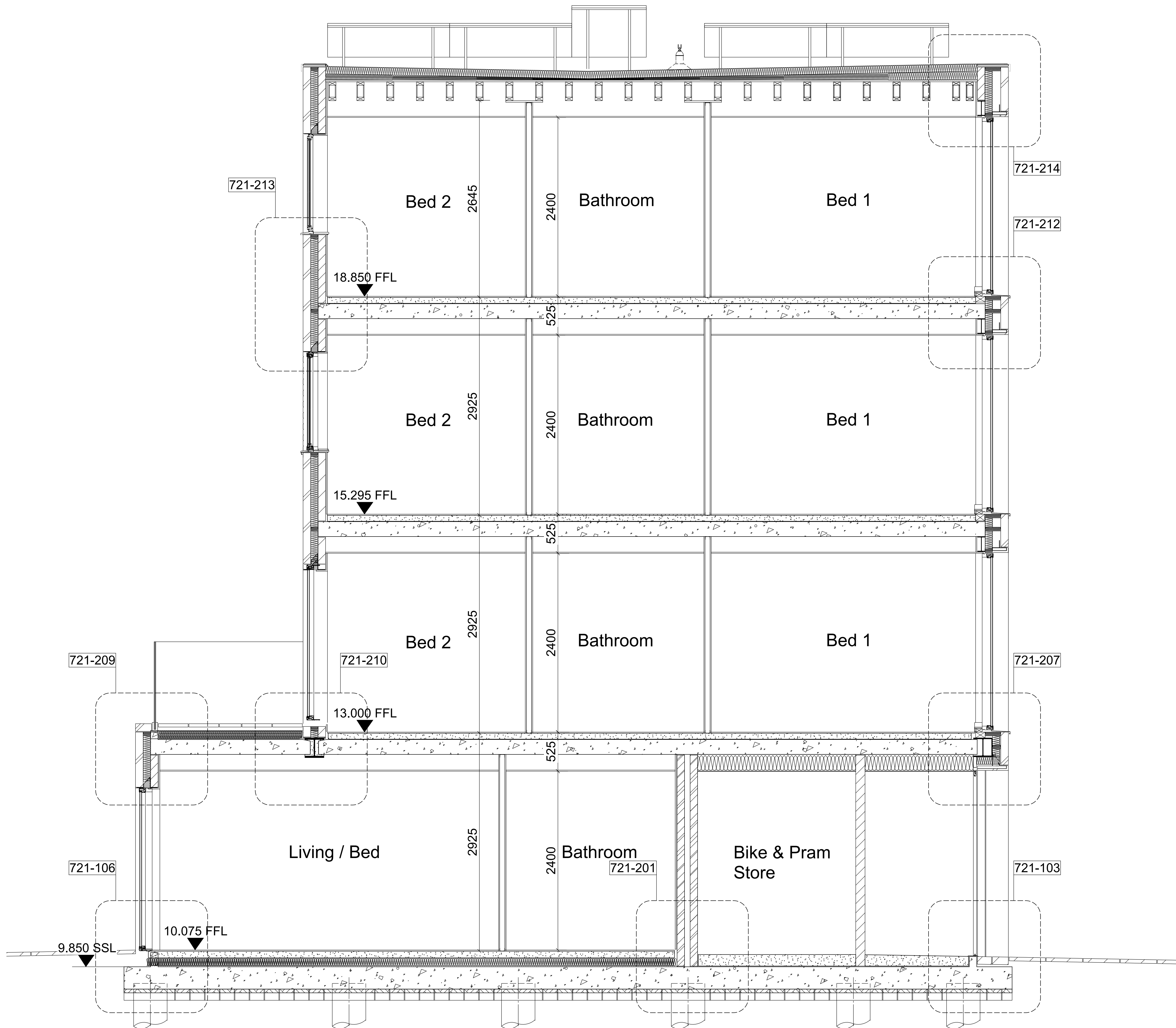
Cross Section East-West between grids G-H Scale 1:50 @ A3
