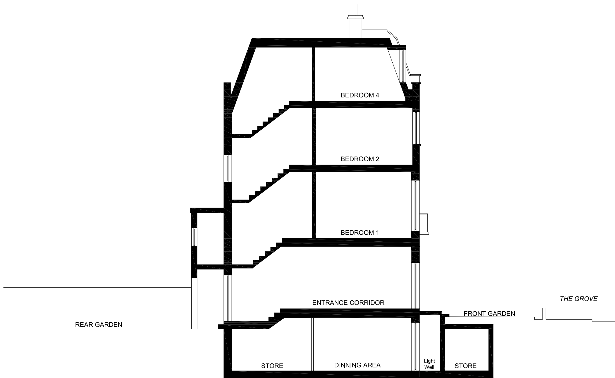
SECTION B-B
