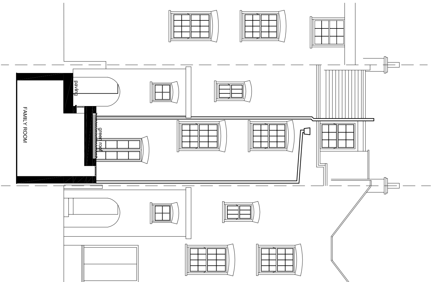
SECTION C-C
