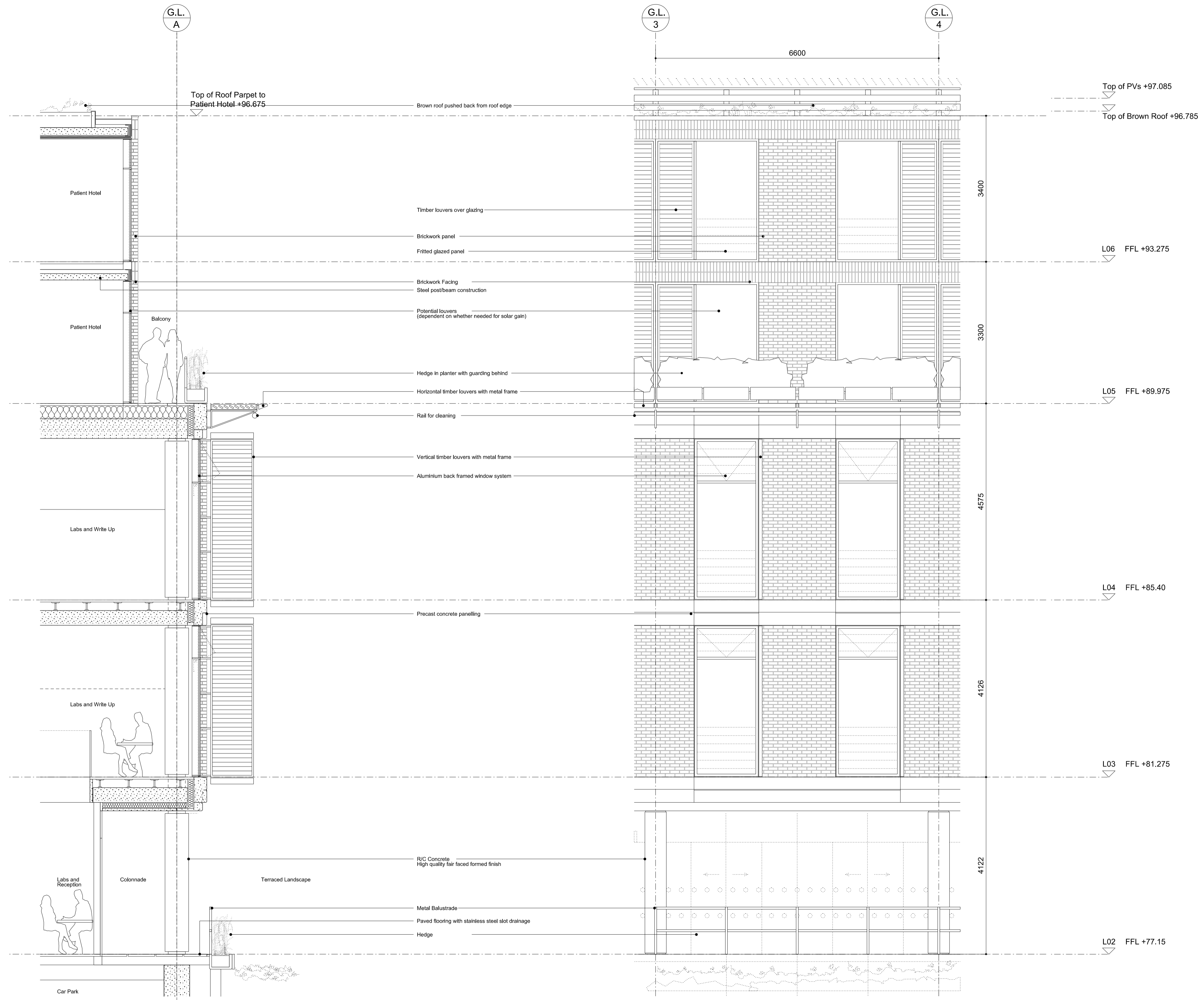
03 Typical Bay Elevation 2150 1:50
