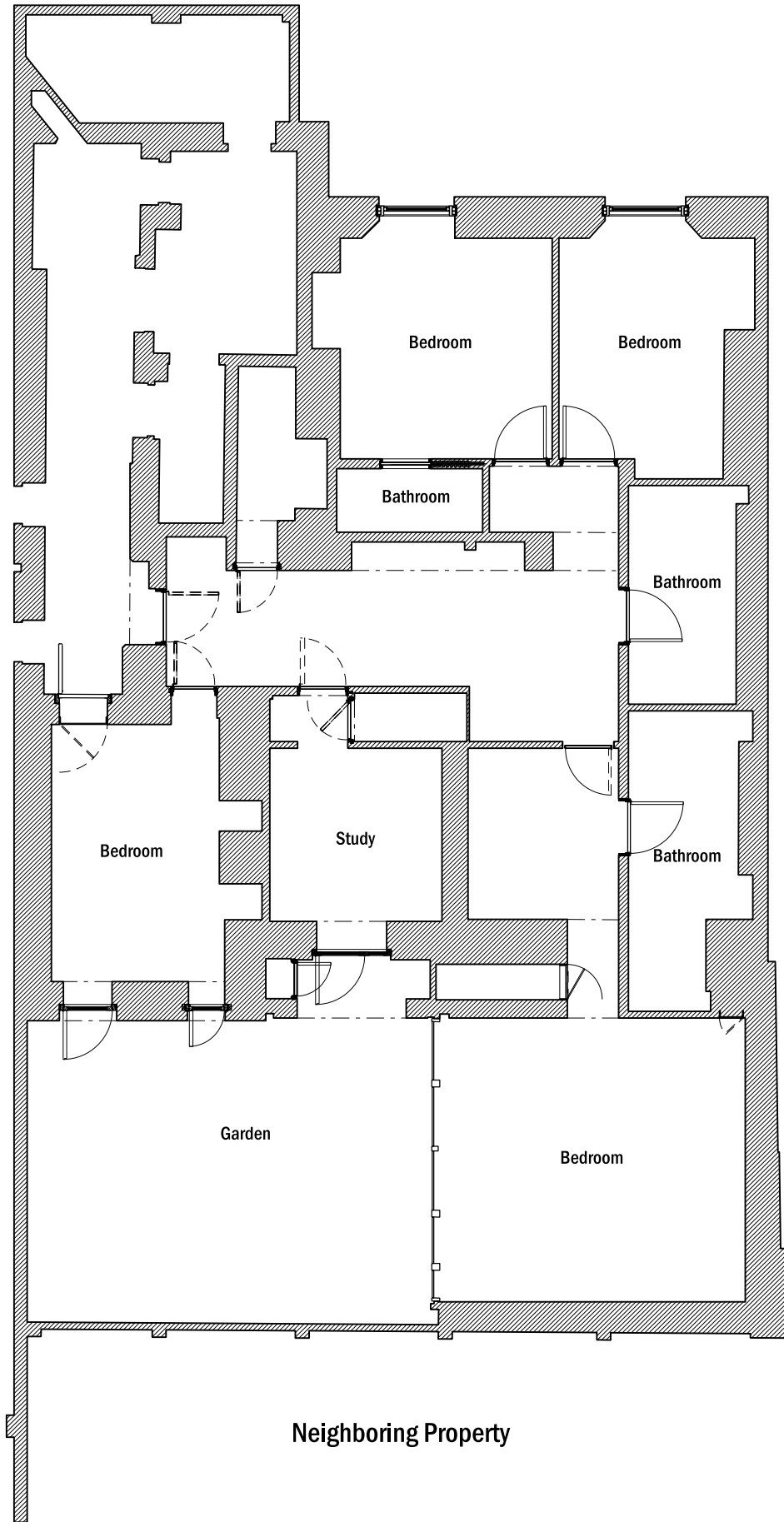
01 As Existing Lower Ground Floor Plan 1:100@A3
