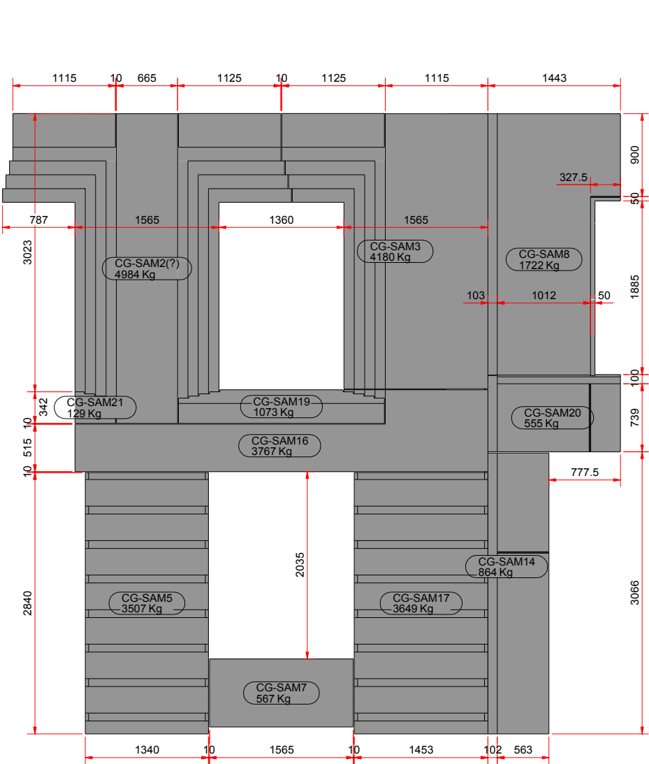
Elevation Bricks Omitted
