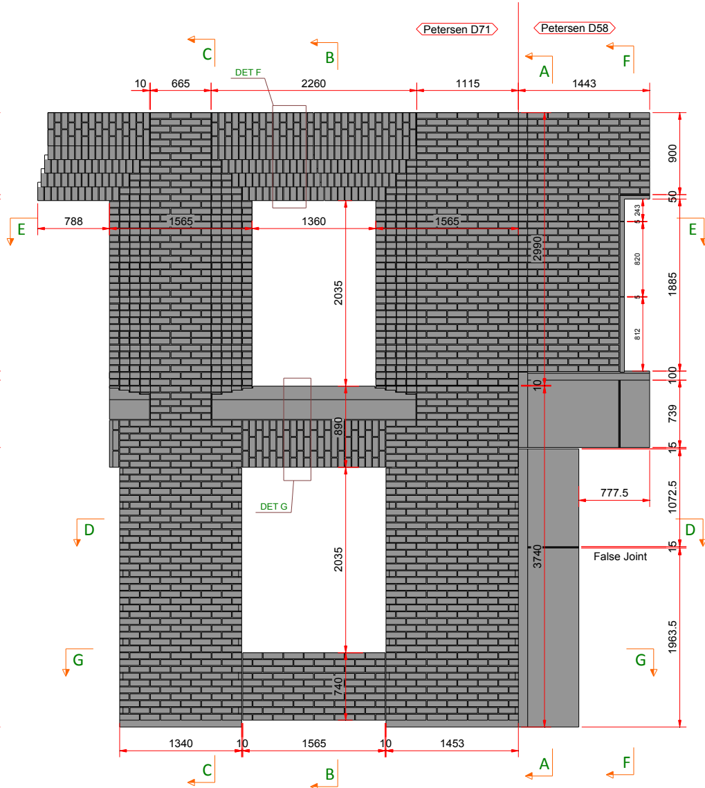
Elevation Bricks Visible
