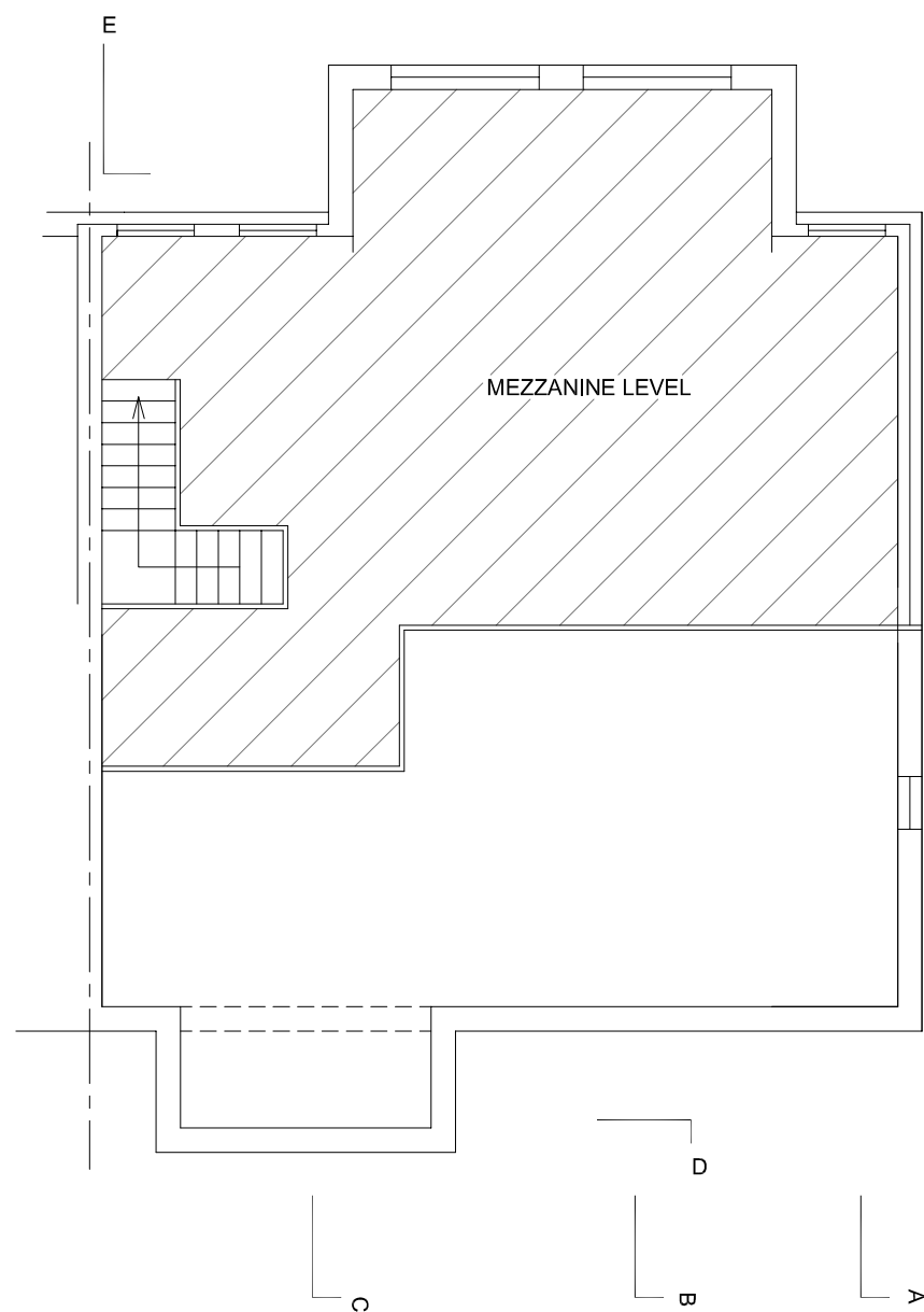
MEZZANINE LEVEL PLAN 58 m2
