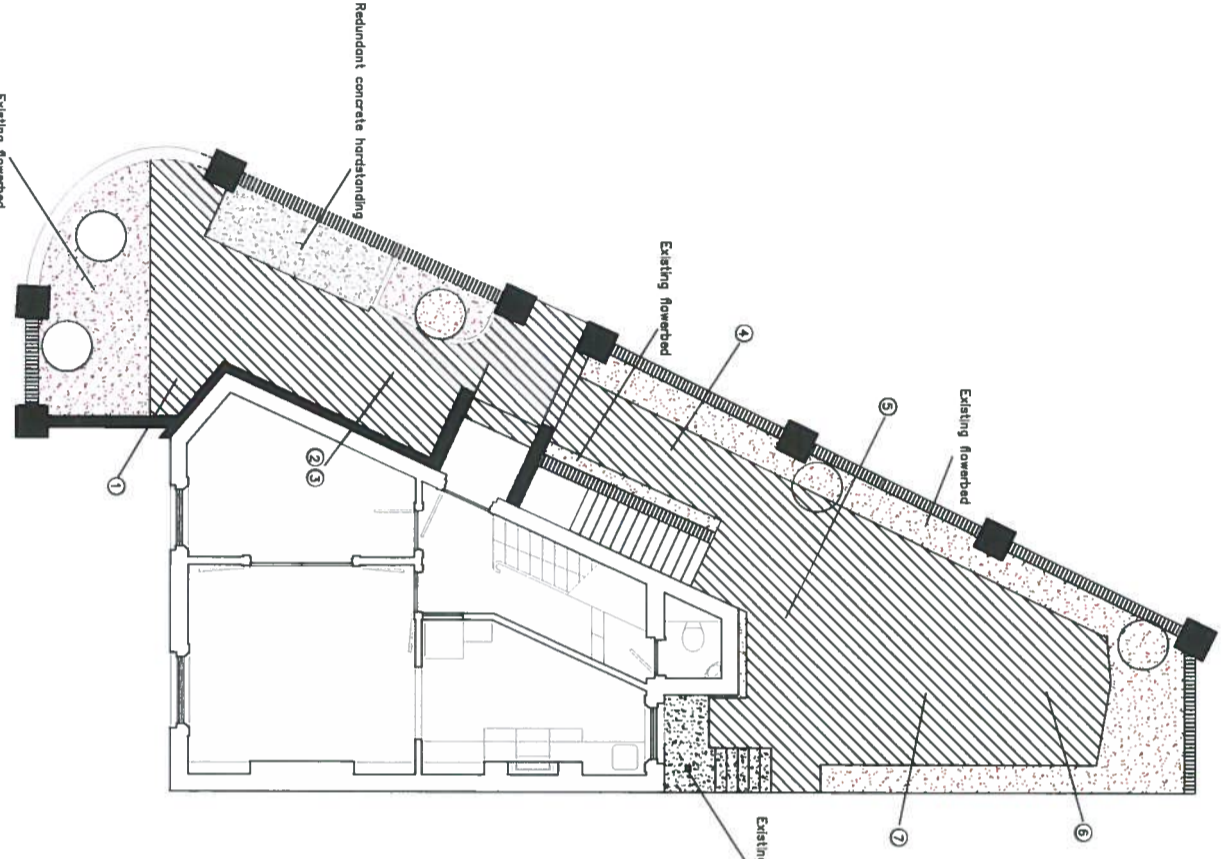
Existing Layout
