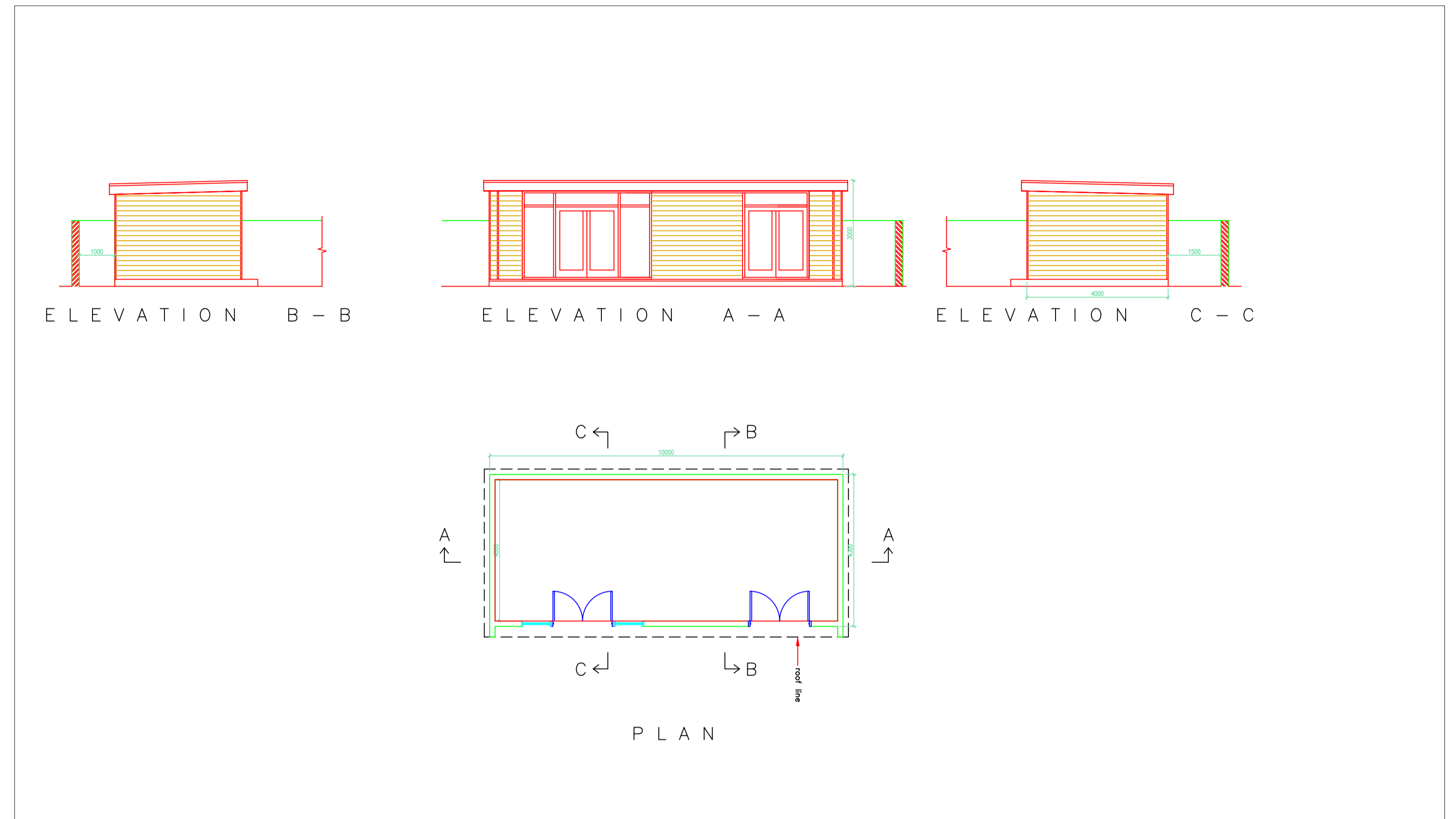
Garden Room Plan & Elevations Scale 1:100
