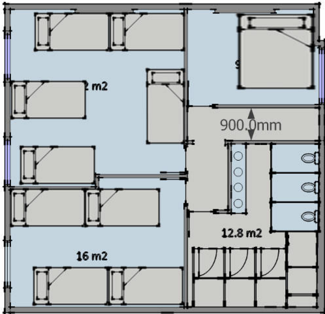
Second Floor: Proposed. Scale 1:50 @ A4
