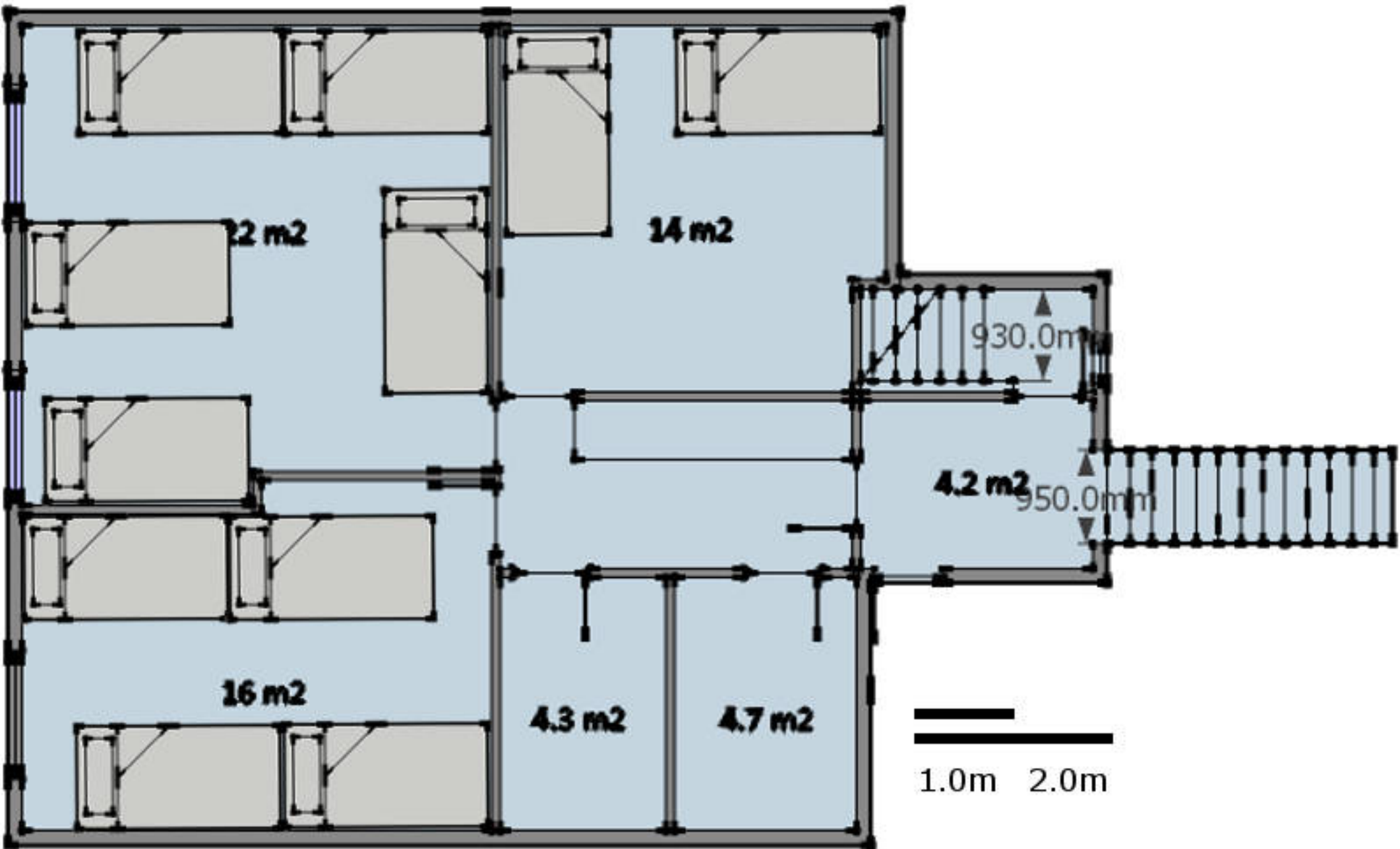
First floor: Proposed. Scale 1:50 @ A4
