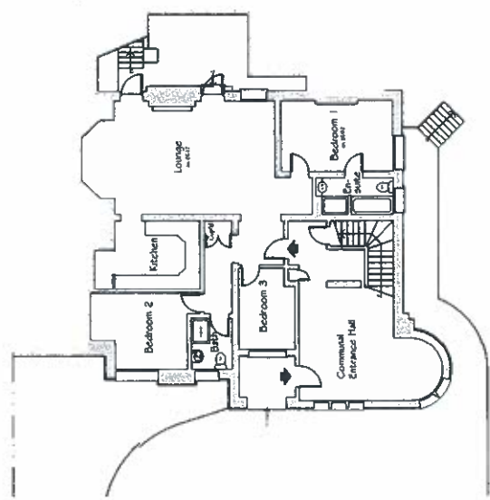
Ground Floor Plan - Flat 1
